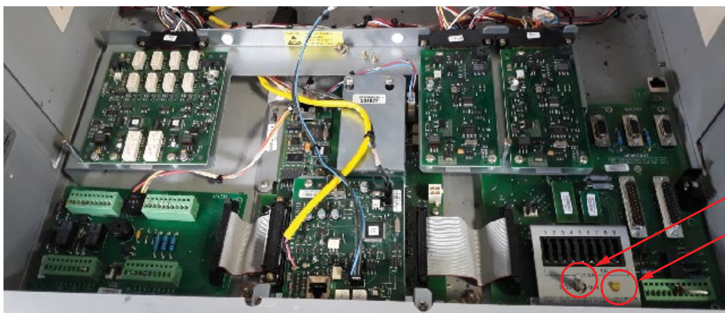
Figure 1.5 Inhibit Switch Location
