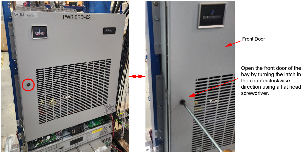
Figure 2.3 Opening of the Front Door
