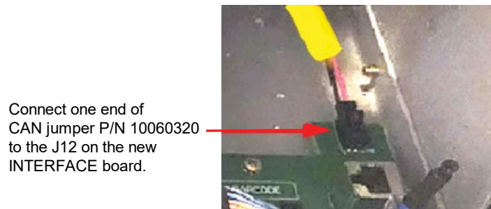
Figure 1.20 Connecting the CAN Jumper P/N 10060320
