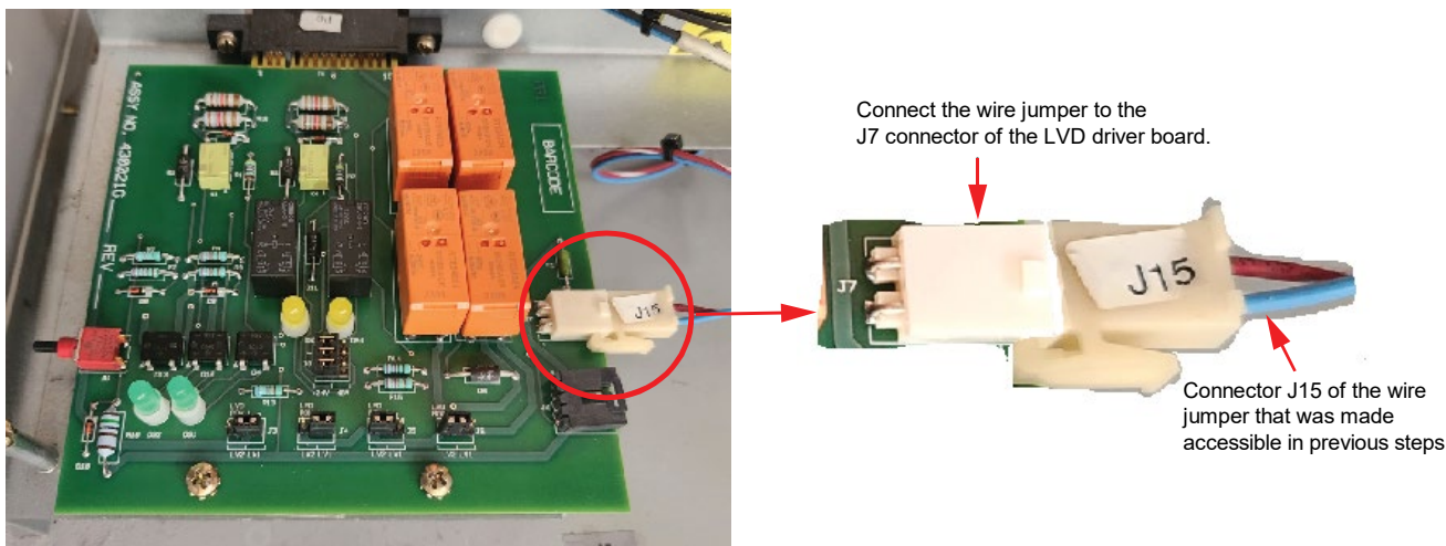
Figure 2.13 Connecting the Wire Jumper
