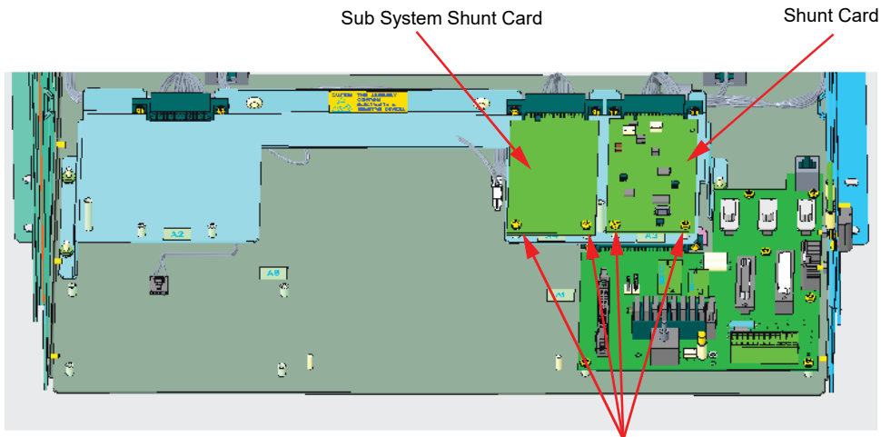
Figure 1.11 Removing the Shunt Cards
