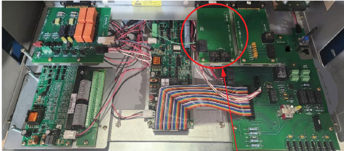
Figure 2.37 Installing CAN INTERFACE Board
