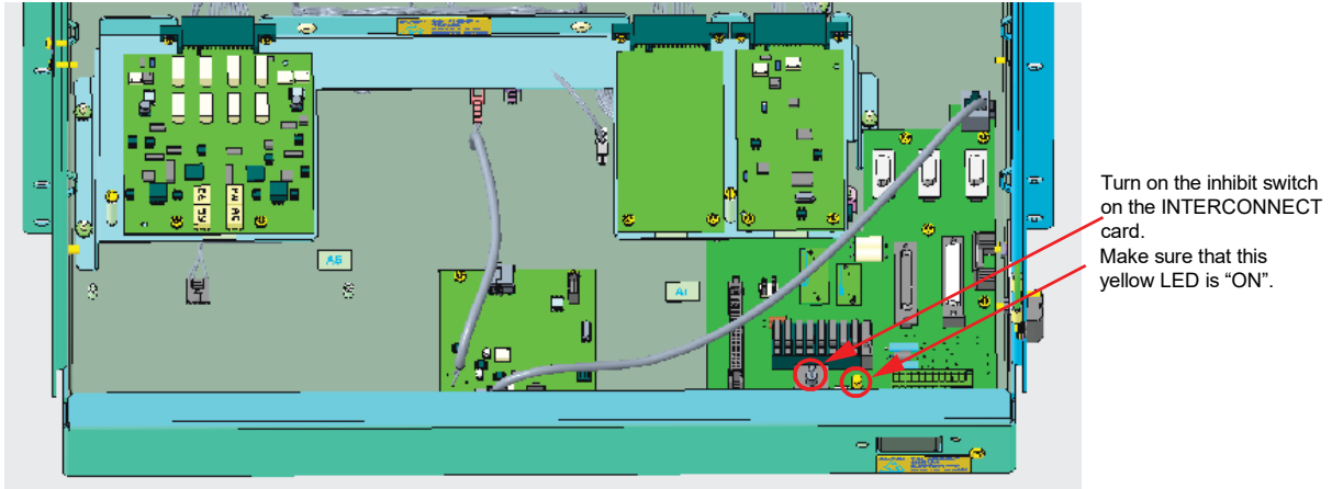
Figure 2.5 The Inhibit Switch Location
