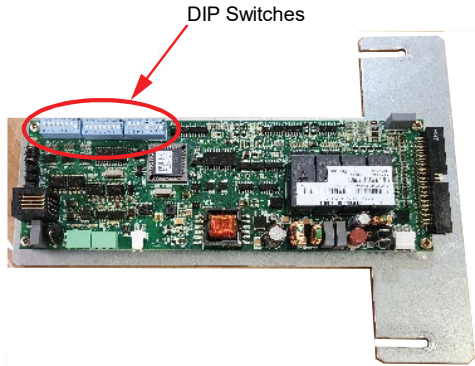
DIP Switches Positions
