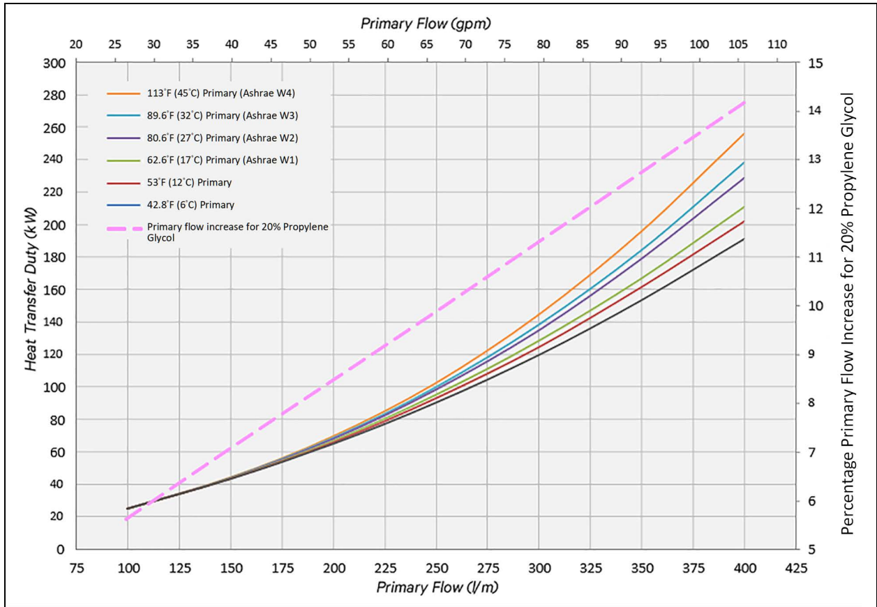
Figure 4.2 Primary Flow/Temperature Graph for 5.4°F (3°C) ATD
