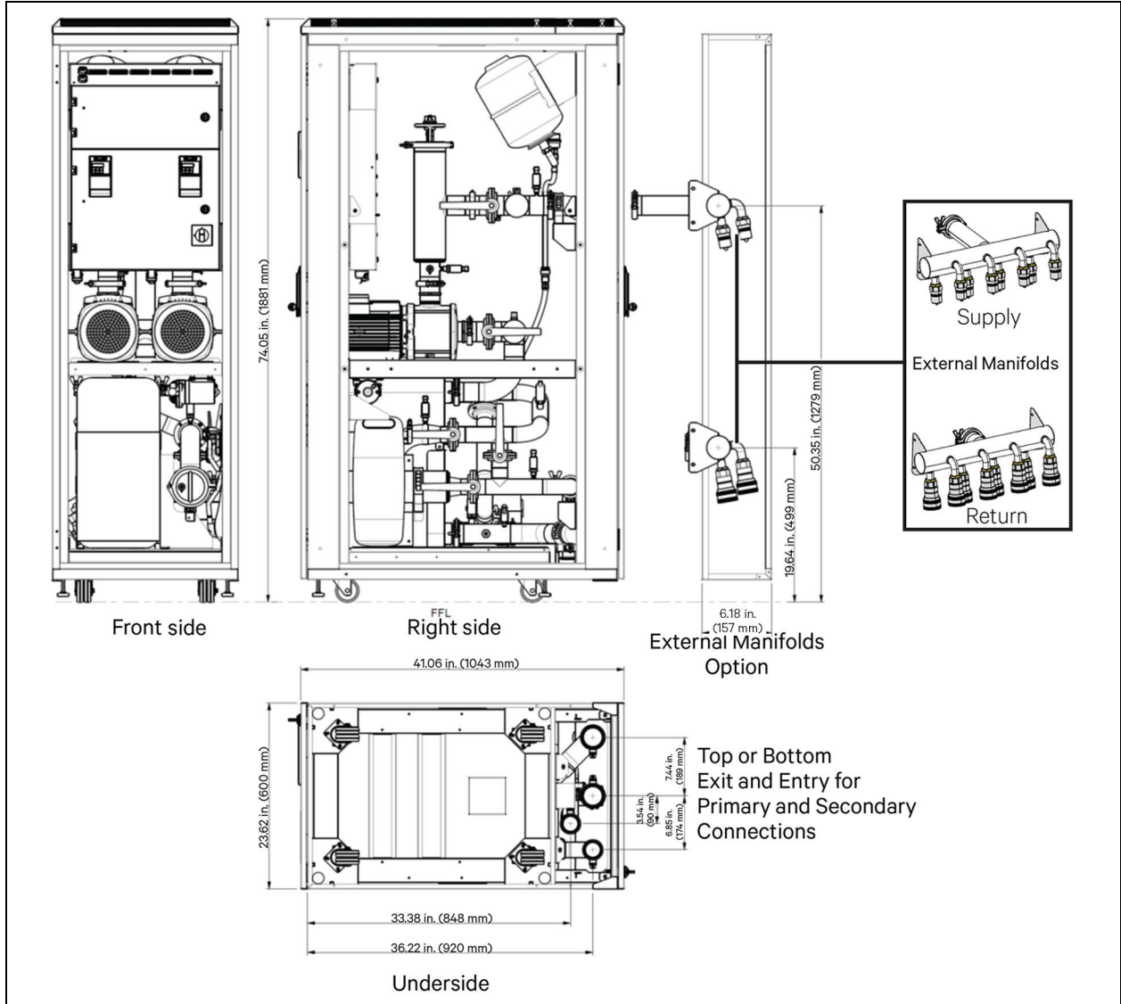
Figure 3.4 Vertiv™ Liebert® XDU450 Cabinet and Piping Dimensions
