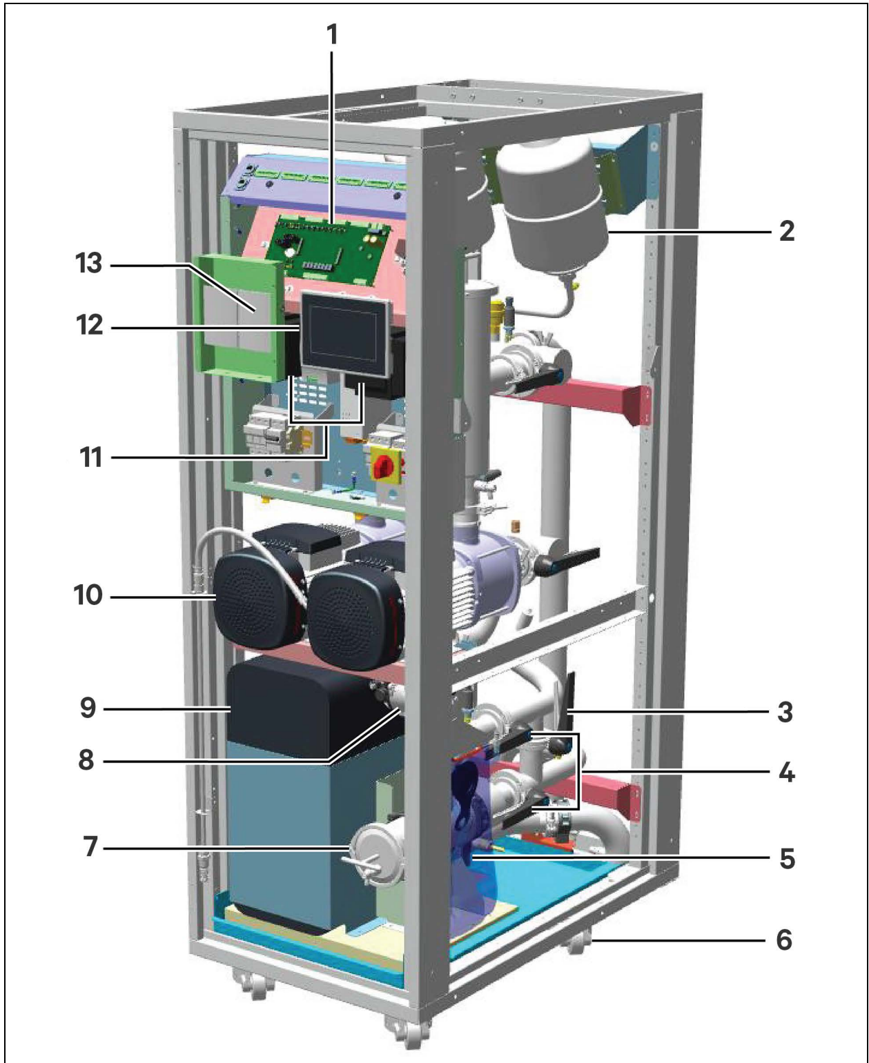
Figure 3.1 Front View of Vertiv™ Liebert® XDU450 (without panels)
