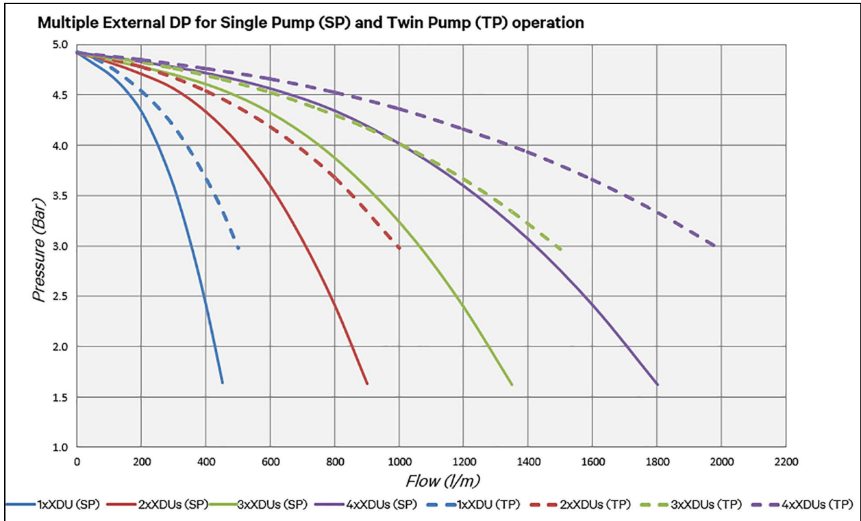
Figure 4.6 Flow/Pressure Graphs for Multiple Units (pumps) in Parallel
