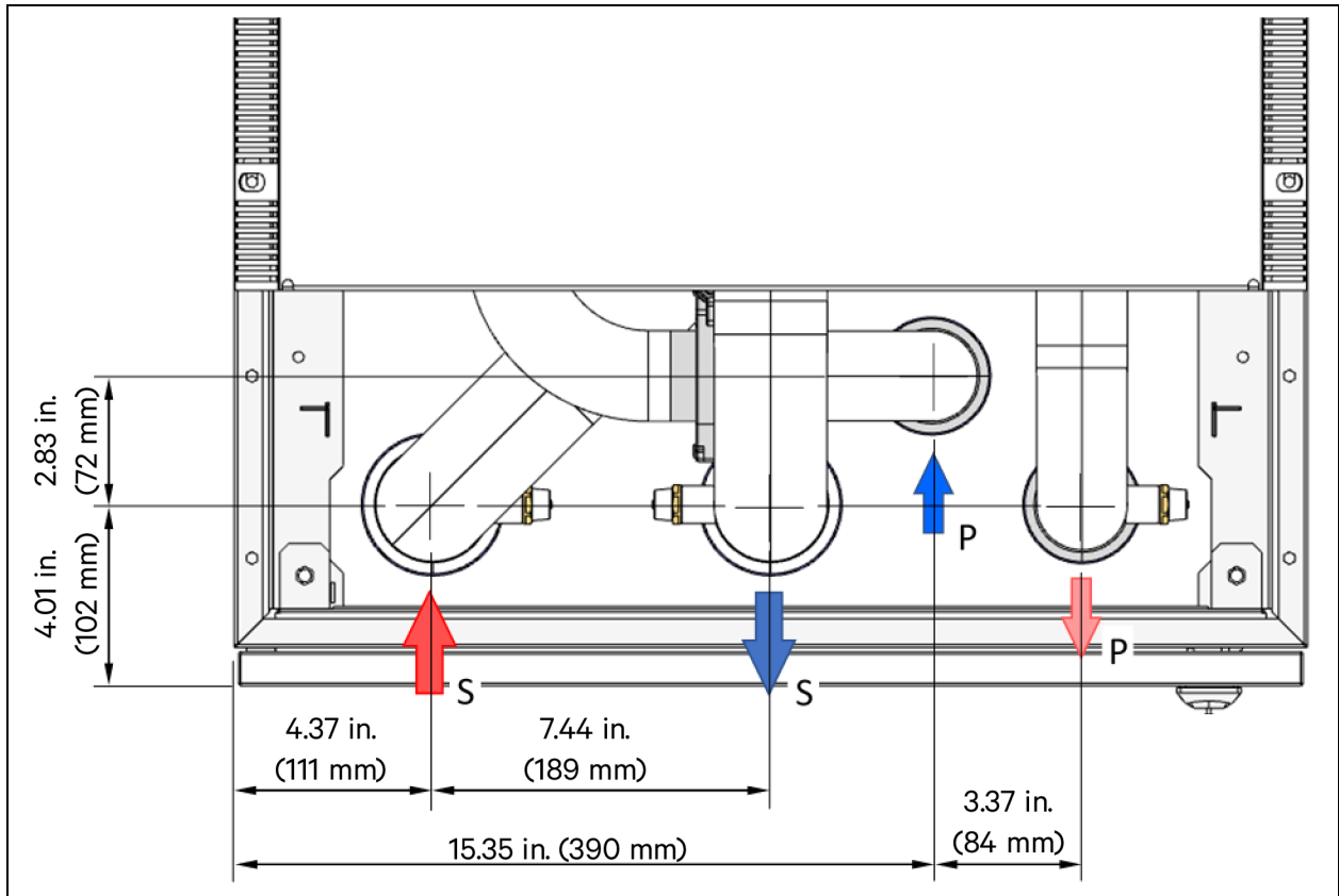
Figure 3.3 Rear Section Showing Primary and Secondary Pipe Connection Locations
