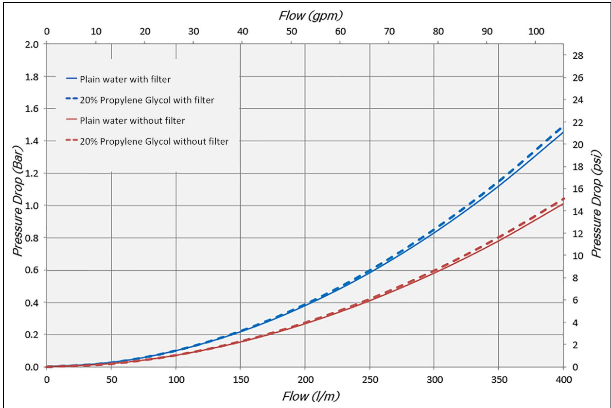
Figure 4.1 Primary Circuit Pressure Drop Graph
