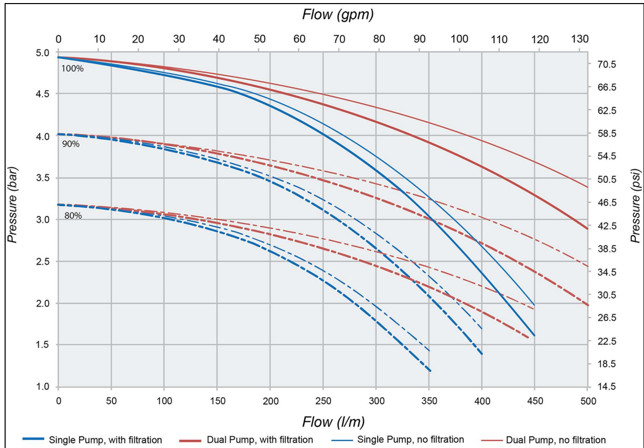
Figure 4.5 Available Secondary External Differential Pressure
