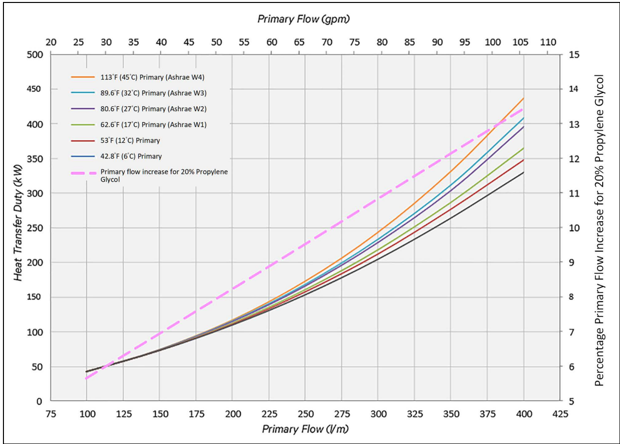
Figure 4.3 Primary Flow/Temperature Graph for 9°F (5°C) ATD
