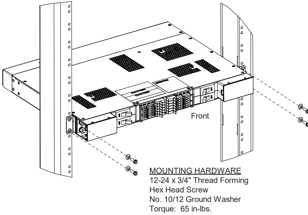
Figure 4.1 Mounting the Distribution Unit in a Relay Rack or a Cabinet Equipment Rack
