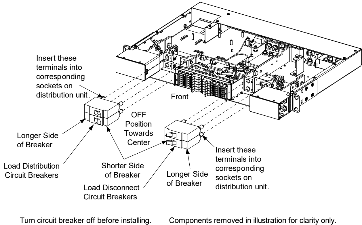
Figure 4.3 Installing Bullet-Nose-Type Load Distribution Circuit Breakers
