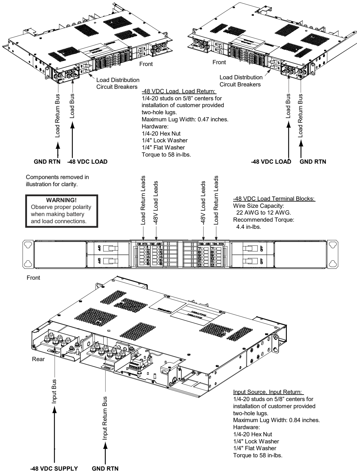
Figure 5.3 Load Distribution Wiring and Input Wiring
