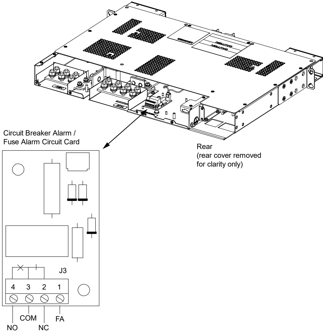
Figure 5.2 External Circuit Breaker / Fuse Alarm Connections
