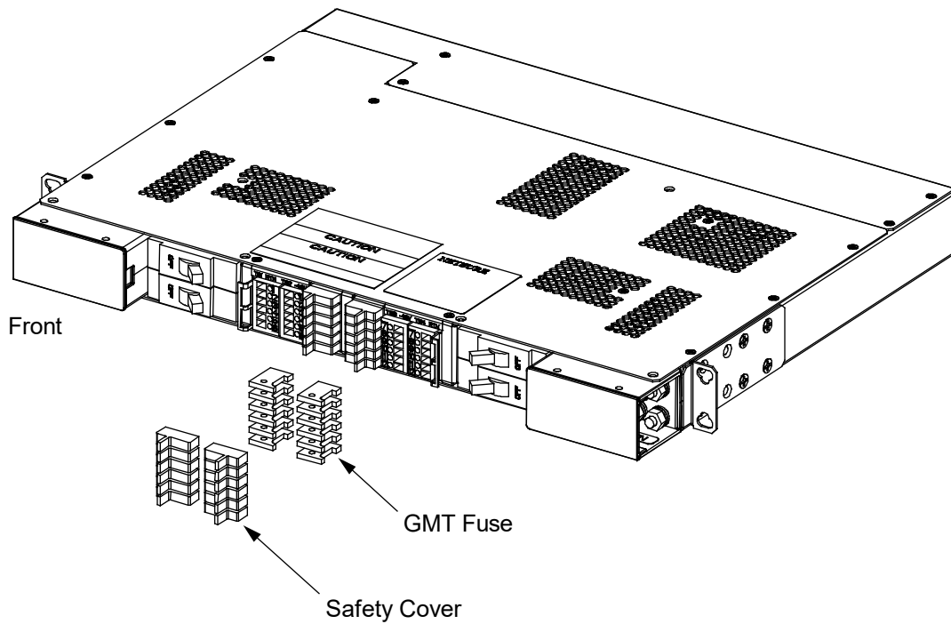
Figure 4.2 Installing GMT Load Distribution Fuses
