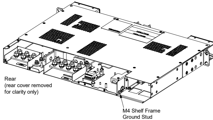
Figure 5.1 Distribution Unit Frame Grounding Connection Points
