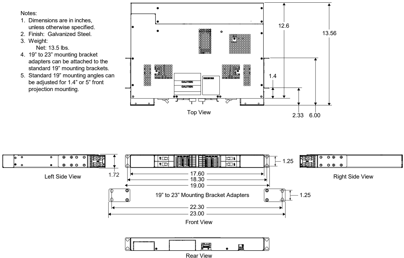
Figure 2.1 Dimensions and Weight
