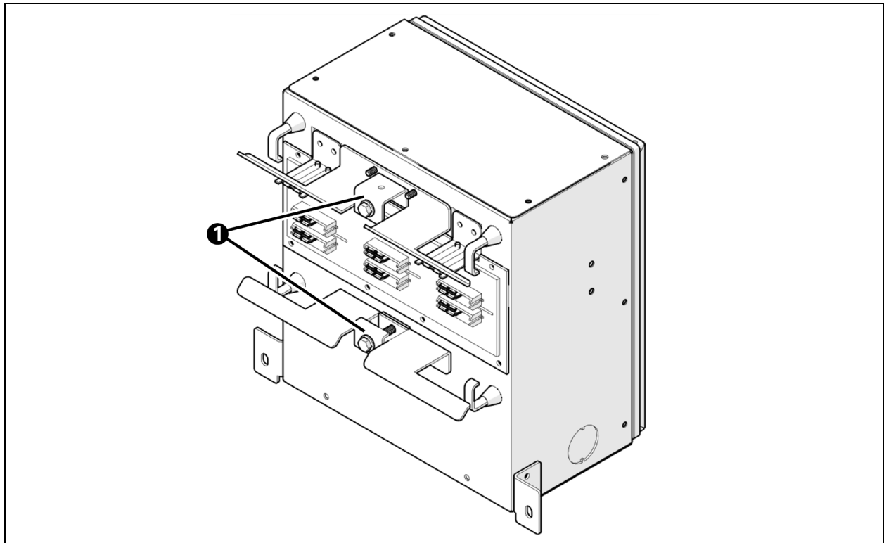
Figure 6.32 Busplug C-Clamps
