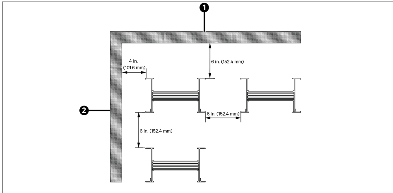
Figure 5.9 Busway Clearances
