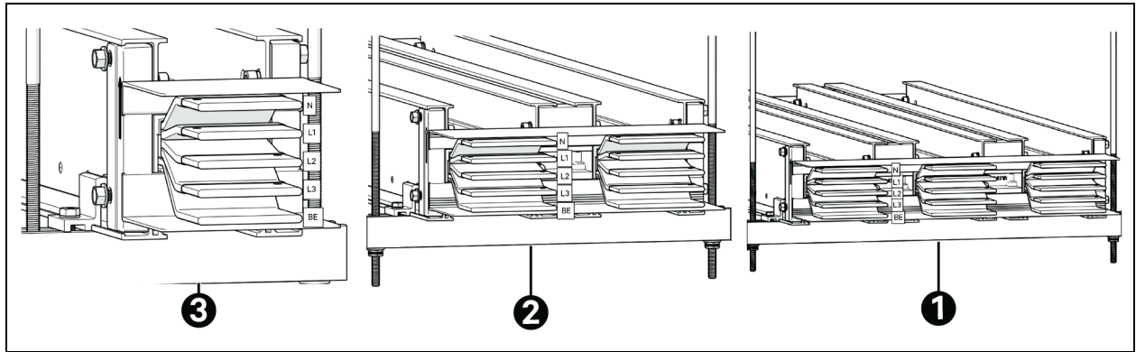
Figure 5.17 Horizontal Flatwise
