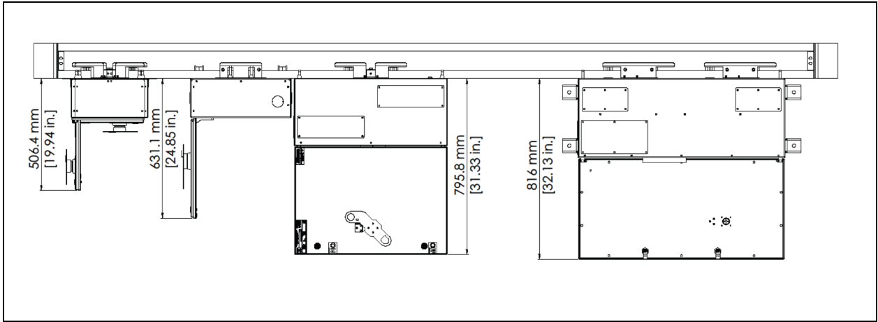
Figure 5.10 Top View of Horizontal Flat Mounted Distribution Busway
