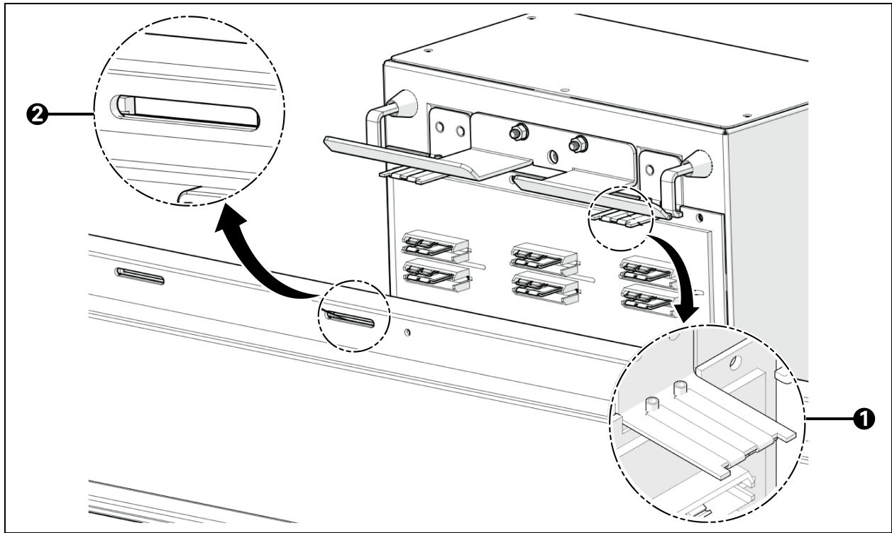
Figure 6.33 Busplug Earth Contacts and Busway Earth Slots
