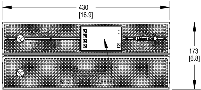
FRONT VIEW FOR DETAIL SEE DRAWING GXE3-DISPLAY
