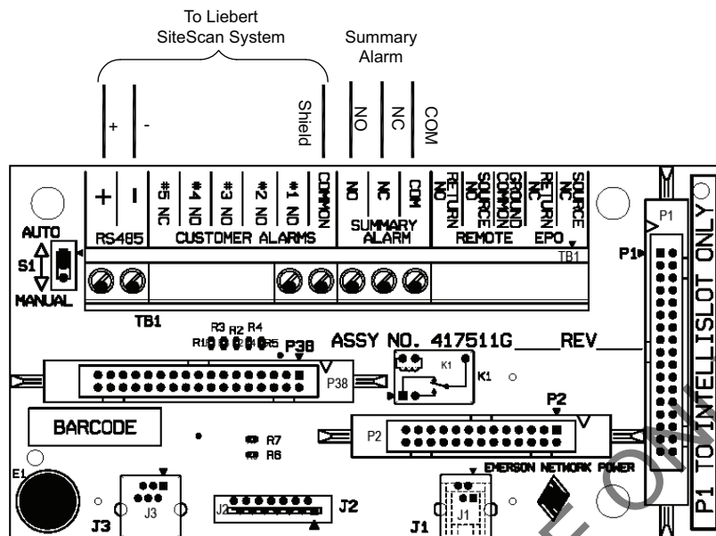
Figure 22 Electrical field connections for Liebert Current Plus and LDMF™ communication and summary alarm
