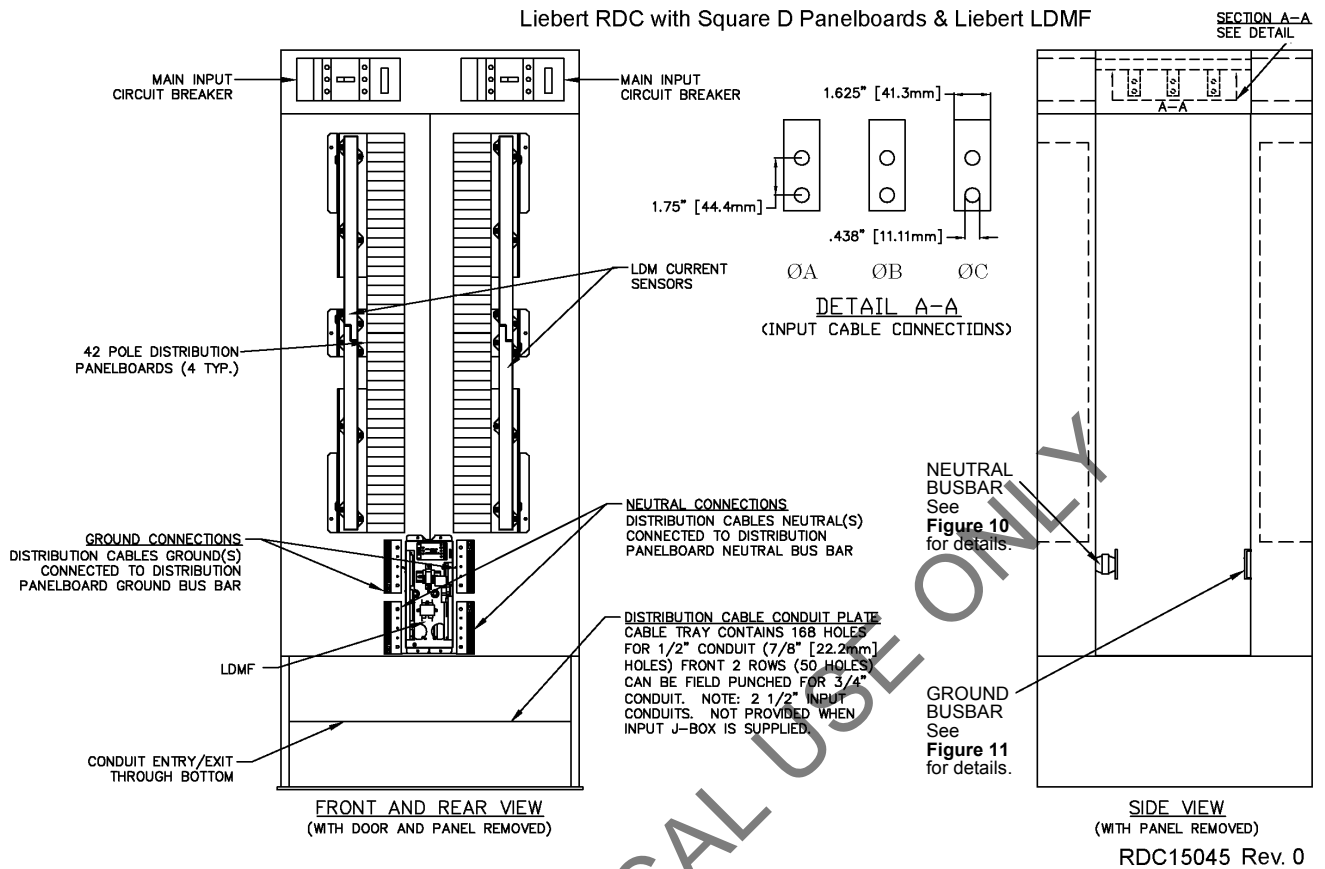
Figure 7 Electrical field connections, one input with Liebert LDMF™
