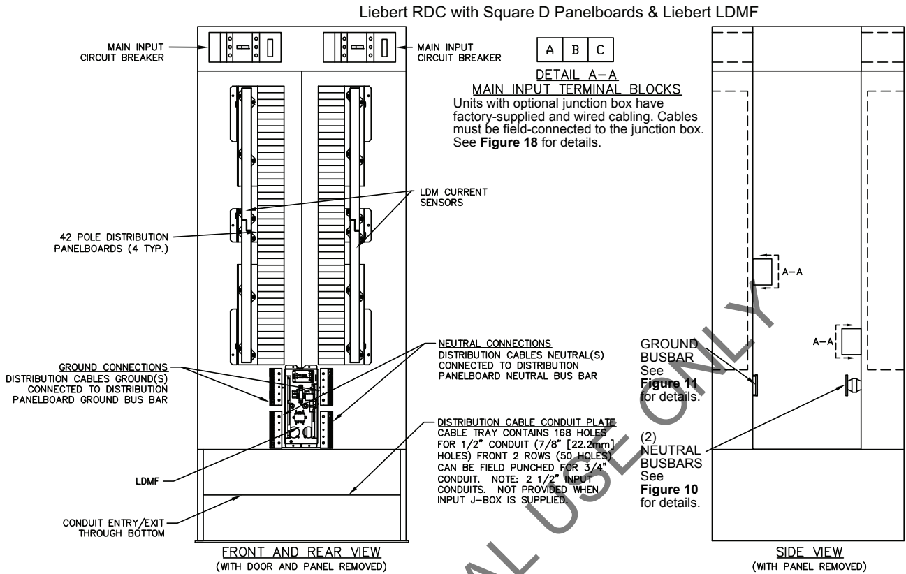
Figure 8 Electrical field connections, two inputs with Liebert LDMF™
