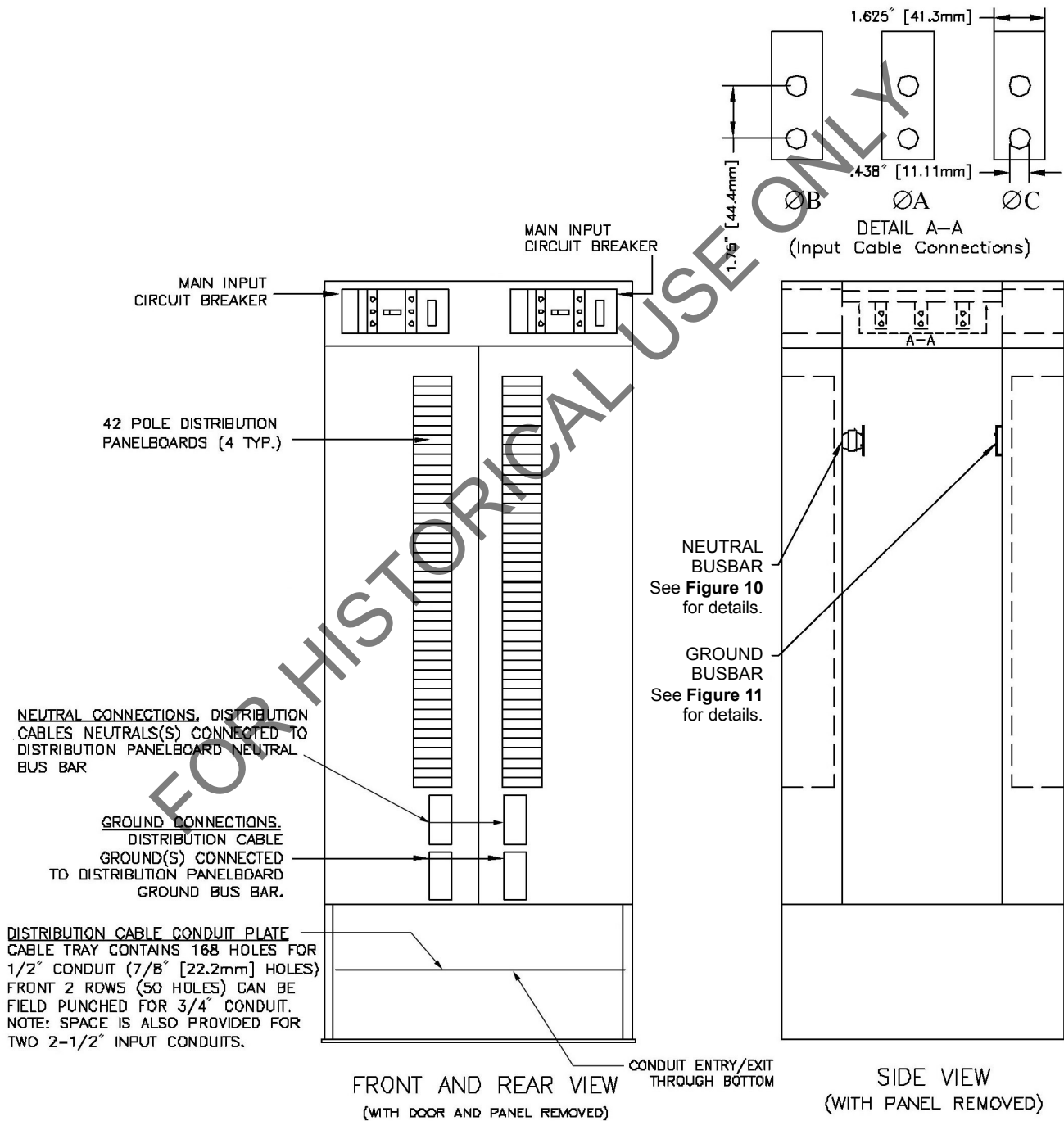
Figure 4 Electrical connection location for single input
