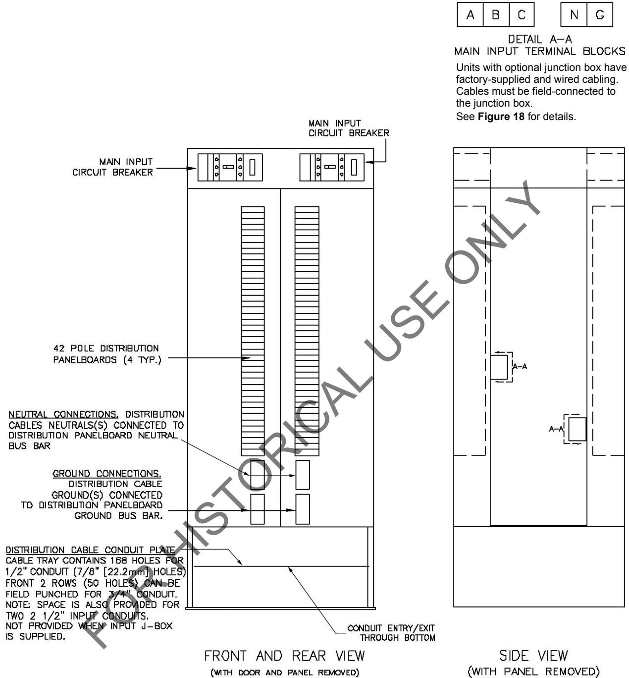
Figure 5 Electrical connection location for two inputs
