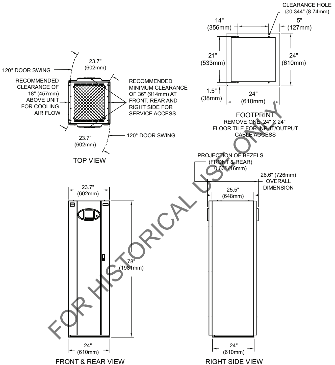
Figure 1 Typical cabinet and floor planning dimension data
