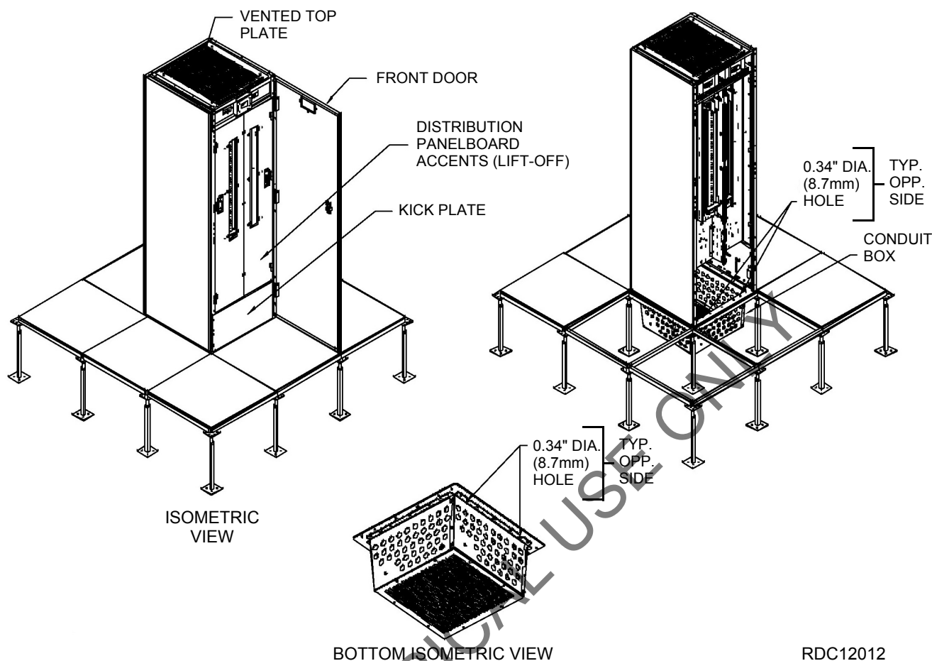
Figure 20 Installation of conduit box
