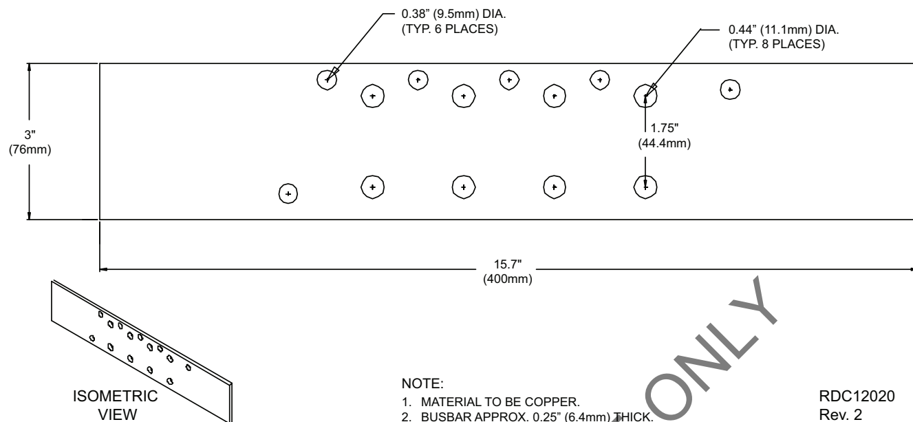
Figure 10 Outline drawing, neutral busbar
