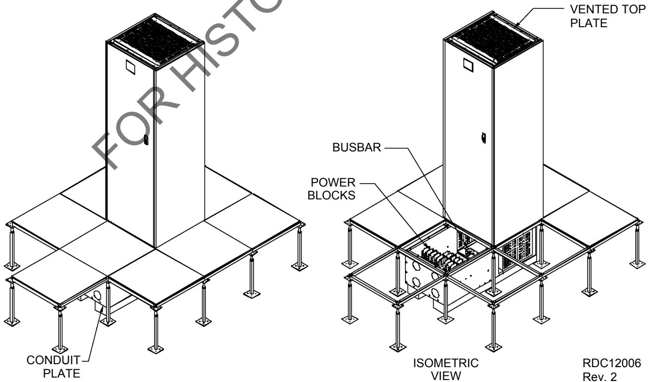
Figure 17 Junction box installation
