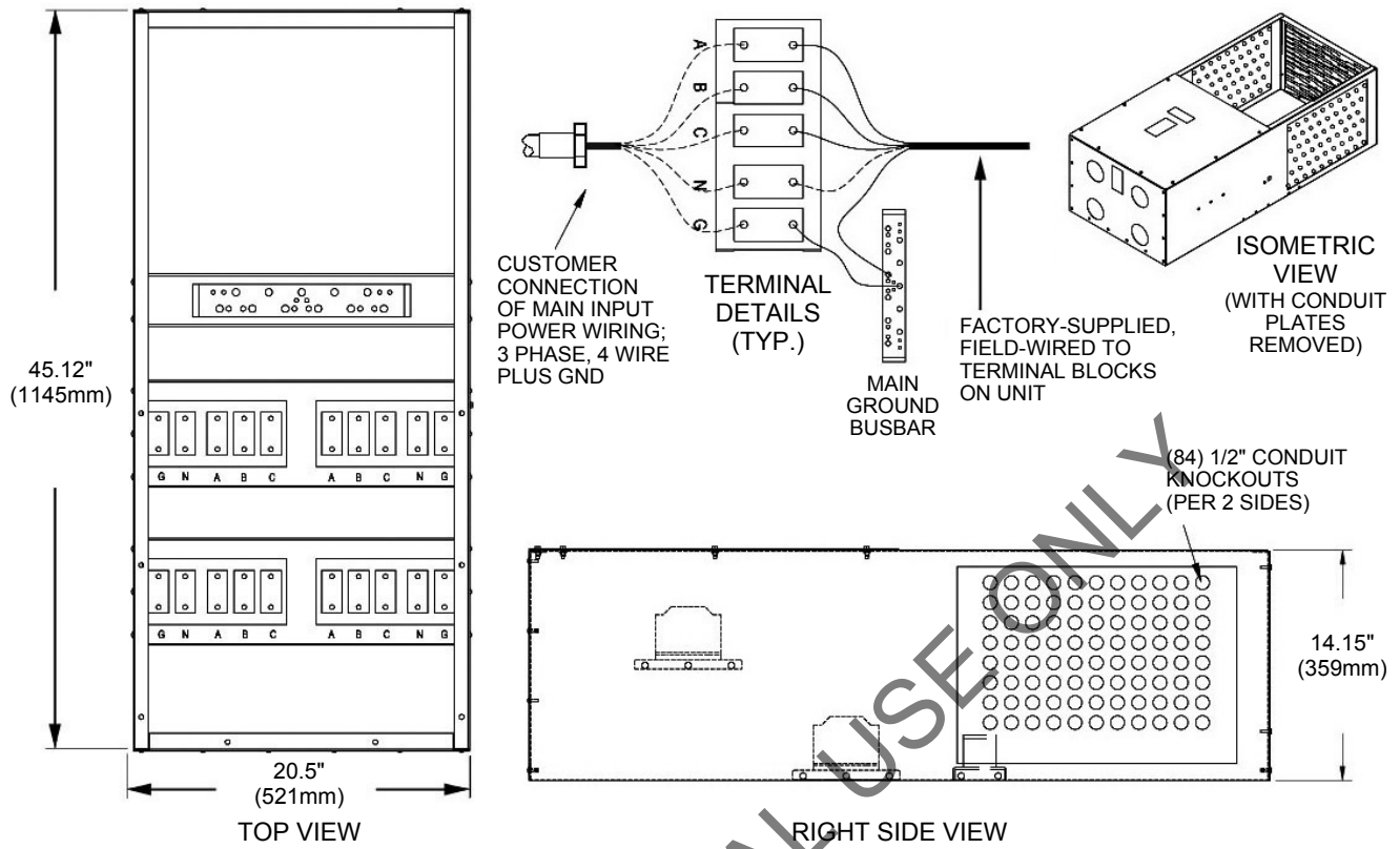
Figure 16 Four input junction box
