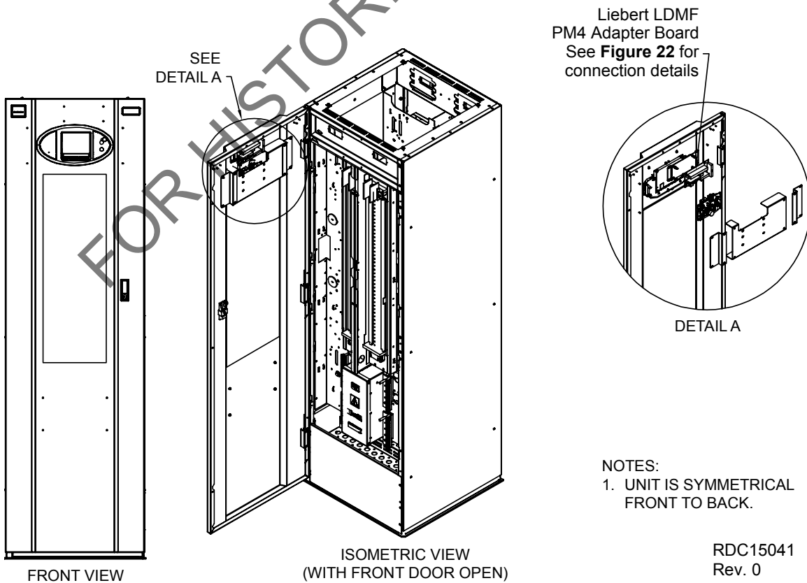
Figure 15 Liebert LDMF adapter board location details
