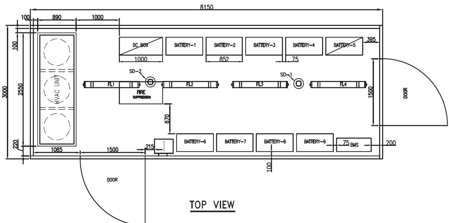
Fig 1: Layout of Prefab Container with Battery Blocks, other Equipment and Vertiv Thermal Management Indoor Unit
