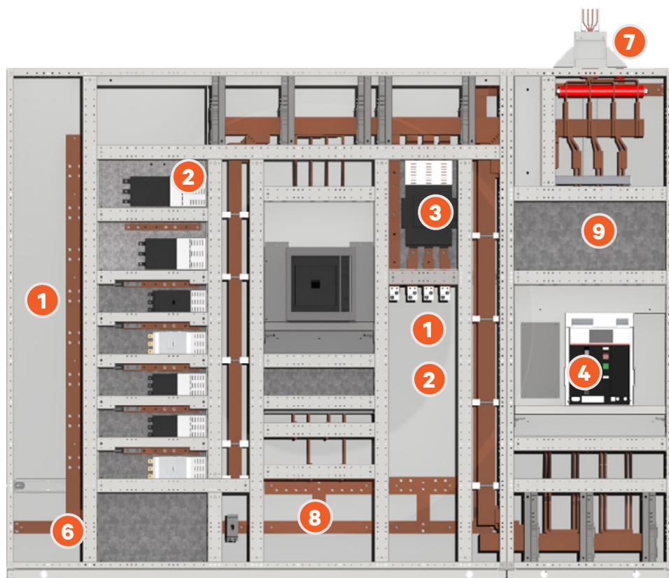
Front Internal View
