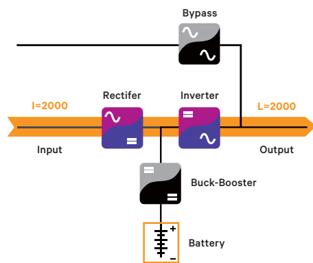
Standard UPS operation (normal operation)
