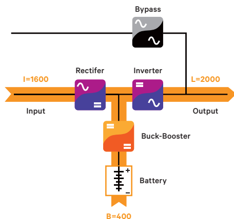
Discharge mode (Partial disconnection)
