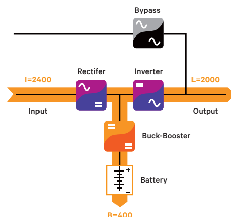
Recharge mode
