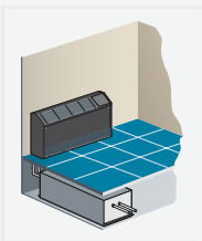
Water/Glycol Cooled Remote. Utilizes an existing water or glycol loop. Condensing unit is located under the raised floor or above the dropped ceiling.
