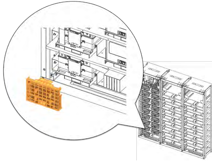
Figure 3-68: Reattach Battery Module #9's Front Cover
