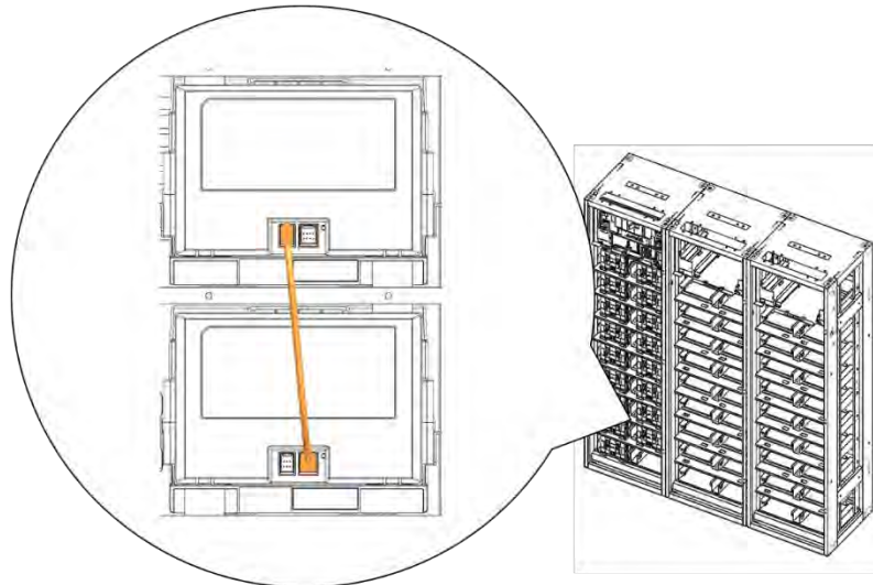
Figure 3-100: Module #7 to Module #8 Signal Cabling
