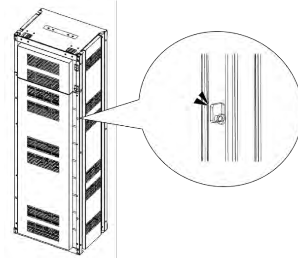
Figure 3-135: Front panel hooks (four)
