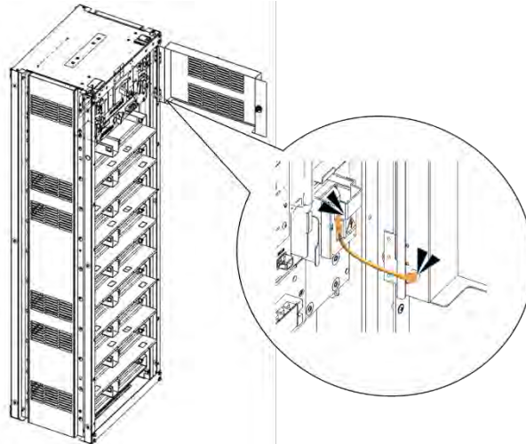
Figure 3-134: Reattaching the earth cable.
