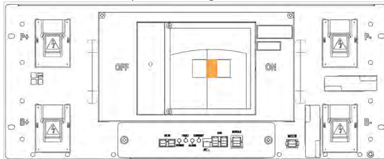
Figure 3-137: MCCB Handle in Trip Position
