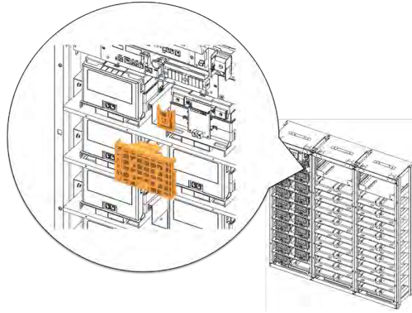
Figure 3-39: Removing the Module #1's Cover and SMU B- Terminal Cover
