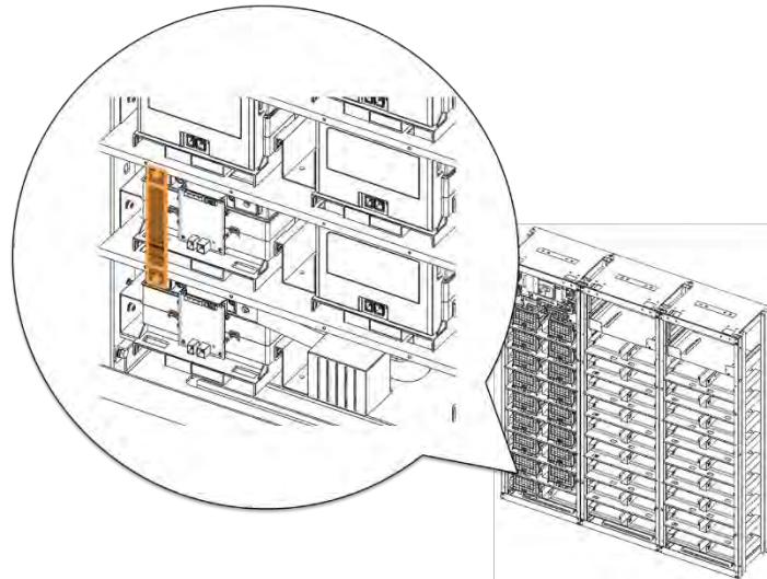
Figure 3-67 Connect Battery Module #9 B+ and Battery Module #10 B-.
