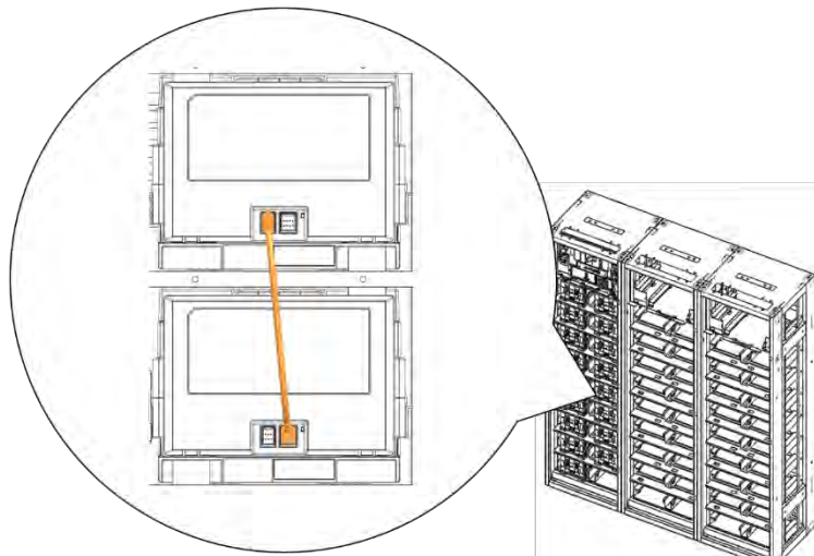
Figure 3-97: Module #4 to Module #5 Signal Cabling
