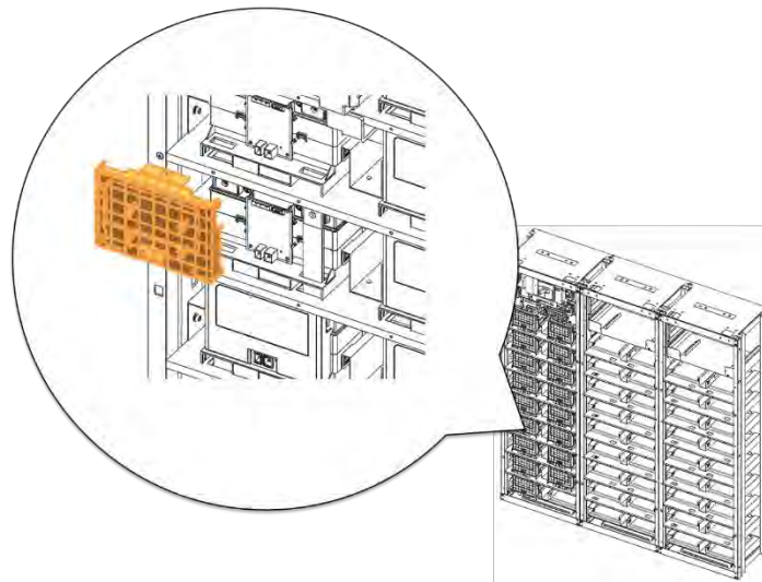
Figure 3-72: Remove Battery Module #12's Front Cover
