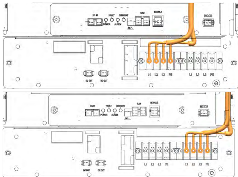
Figure 3-124: SMPS Assembly 3 Phase Type B - AC Input Terminals with Cables Attached
