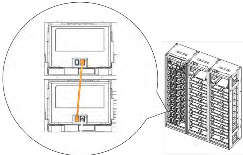
Figure 3-103: Module #10 to Module #11 Signal Cabling
