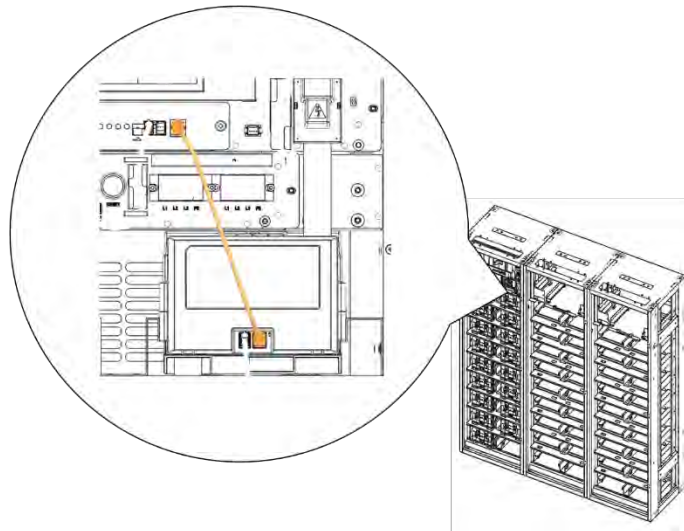
Figure 3-93: SMU to Module #1 Signal Cable
