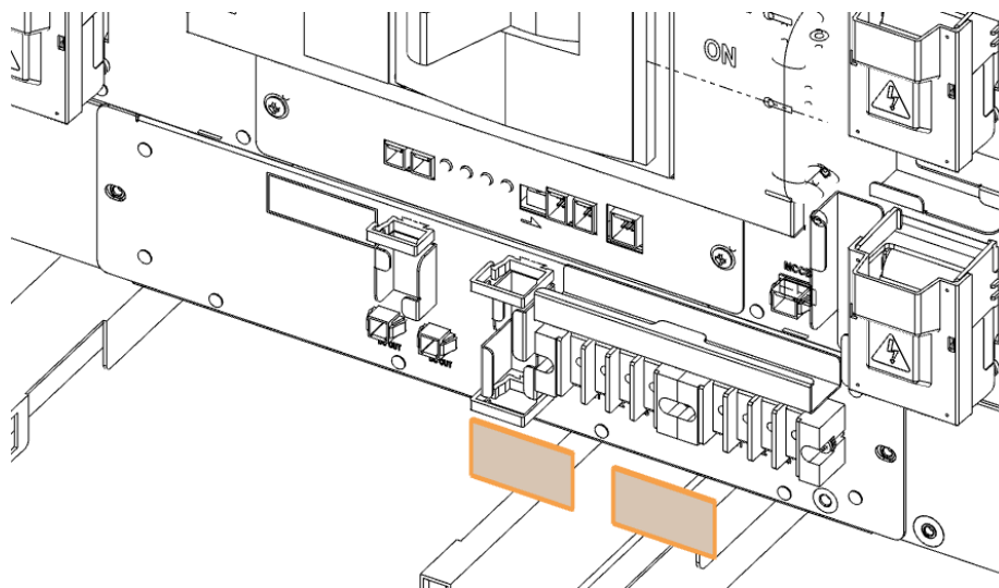
Figure 3-120: AC Input Terminals of SMPS Assembly 3 Phase Type B
