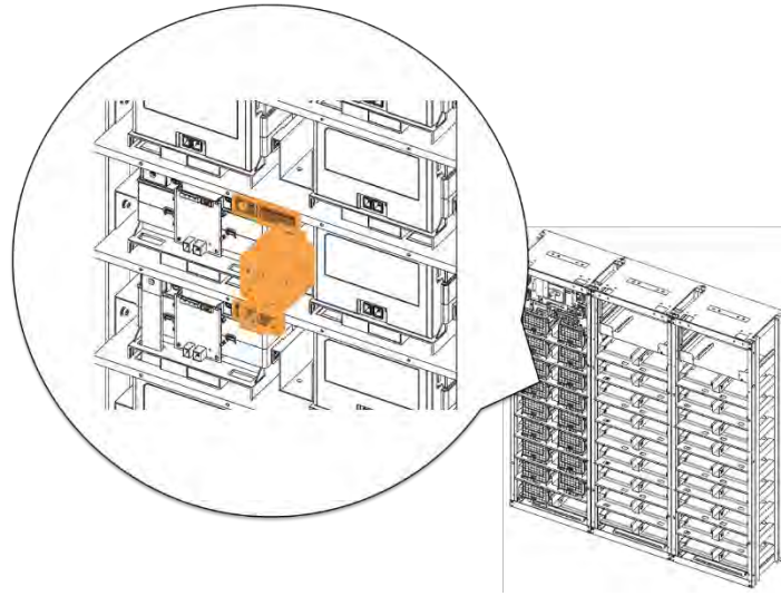
Figure 3-82: Connect Battery Module #14 B+ and Battery Module #15 B-.
