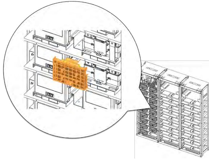
Figure 3-53: Reattach Battery Module #4's Front Cover
