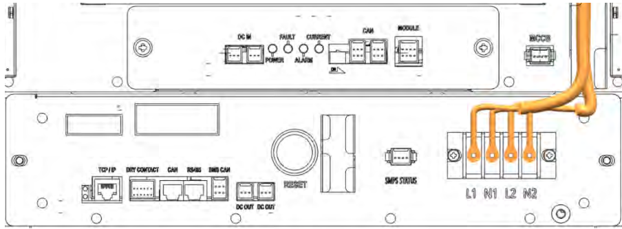
Figure 3-125: SMPS Assembly 1 Phase Type A - AC Input Terminals with Cables Attached
