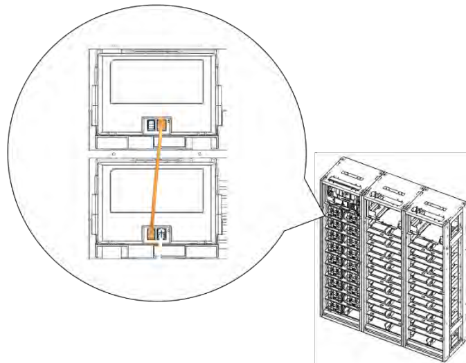
Figure 3-109: Module #16 to Module #17 Signal Cabling
