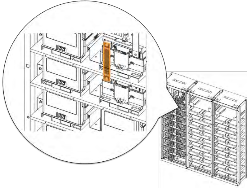
Figure 3-43: Connect Battery Module #1 B+ and Battery Module #2 B-.
