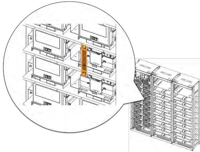
Figure 3-50: Reattach Battery Module #3's Front Cover
