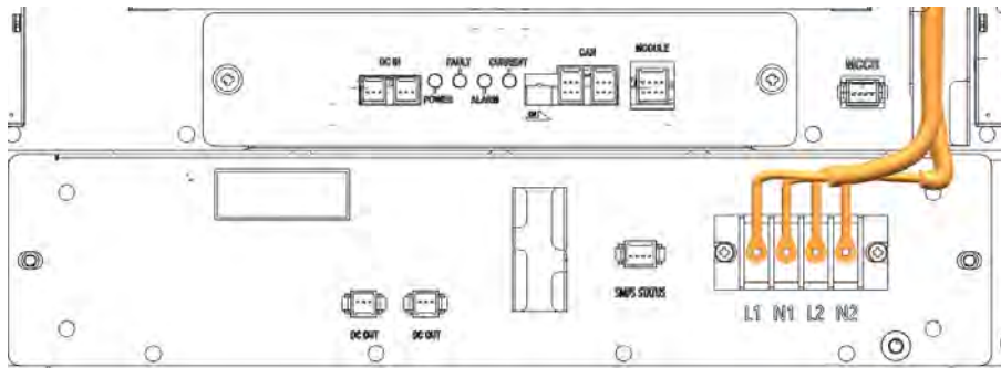
Figure 3-126: SMPS Assembly 1 Phase Type B - AC Input Terminals with Cables Attached
