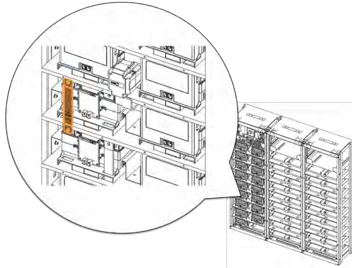
Figure 3-73: Connect Battery Module #11 B+ and Battery Module #12 B-.
