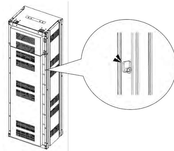
Figure 3-6: Front panel hooks (four)
