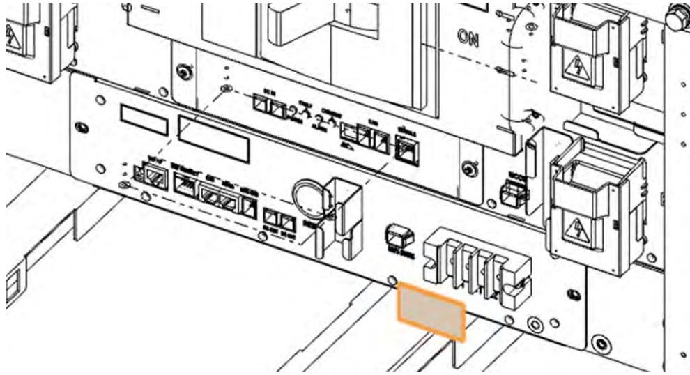
Figure 3-121: AC Input Terminals of SMPS Assembly 1 Phase Type A
