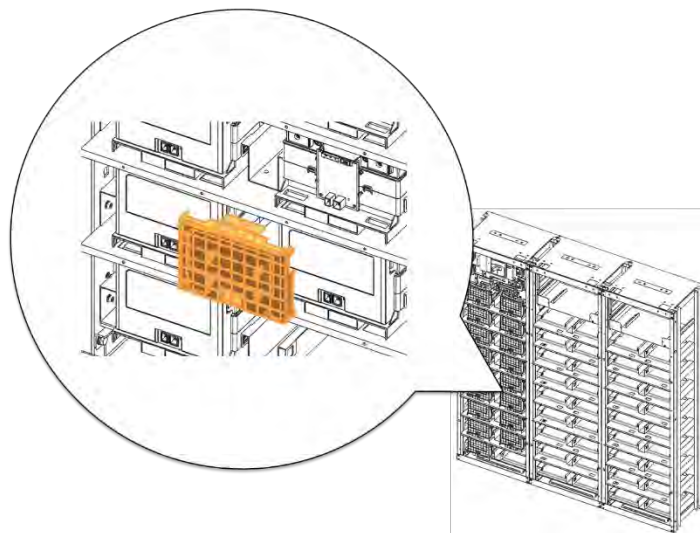
Figure 3-57: Remove Battery Module #7's Front Cover
