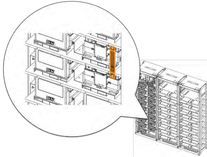
Figure 3-58: Connect Battery Module #6 B+ and Battery Module #7 B-
