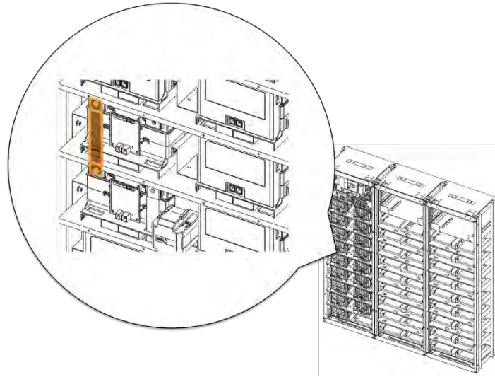
Figure 3-79: Connect Battery Module #13 B+ and Battery Module #14 B-.
