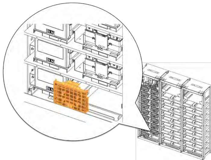
Figure 3-60: Remove Battery Module #8's Front Cover
