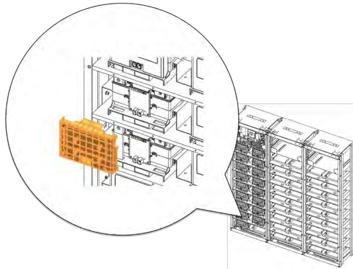
Figure 3-69: Remove Battery Module #11's Front Cover
