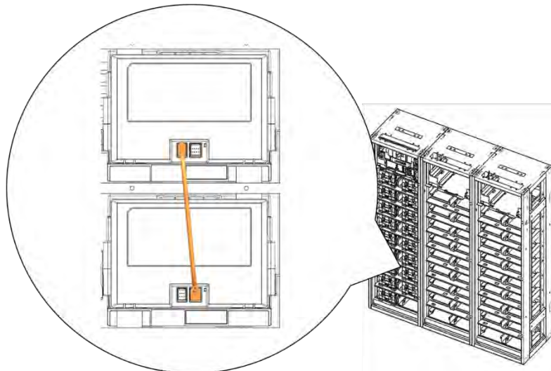
Figure 3-98: Module #5 to Module #6 Signal Cabling
