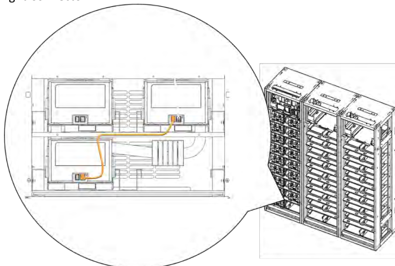
Figure 3-101: Module #8 to Module #9 Signal Cabling
