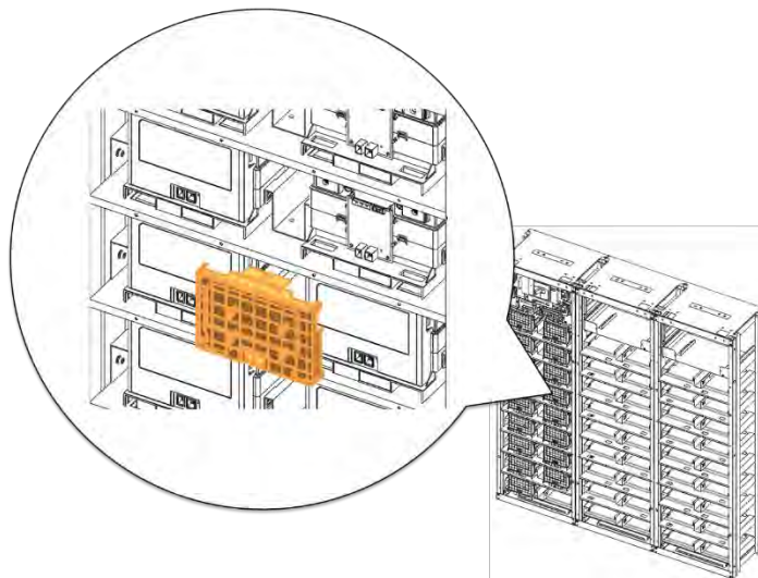
Figure 3-48: Remove Battery Module #4's Front Cover
