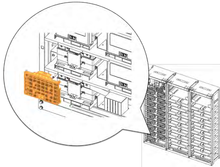
Figure 3-66: Remove Battery Modules #10's Front Cover
