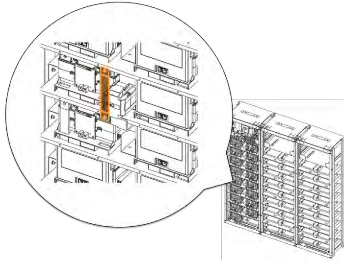
Figure 3-76: Connect Battery Module #12B+ and Battery Module #13 B-.
