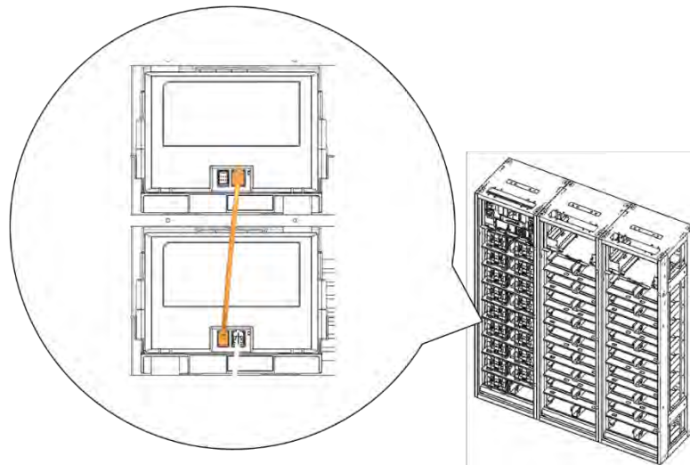
Figure 3-105: Module #12 to Module #13 Signal Cabling
