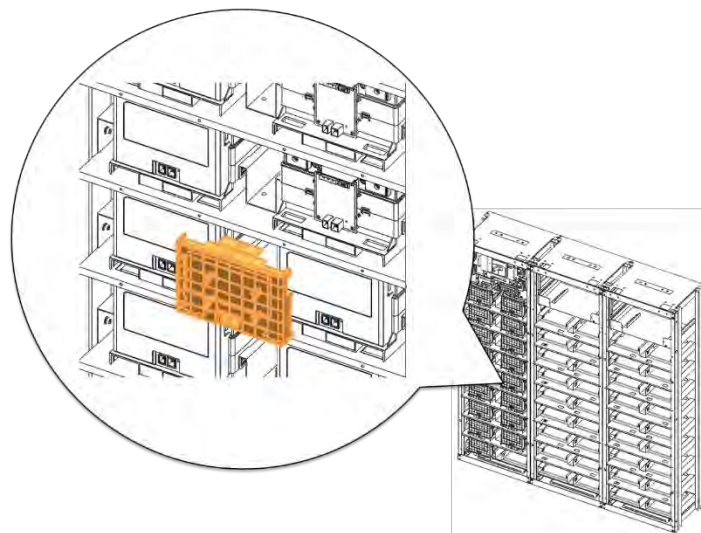
Figure 3-51: Remove Battery Module #5's Front Cover
