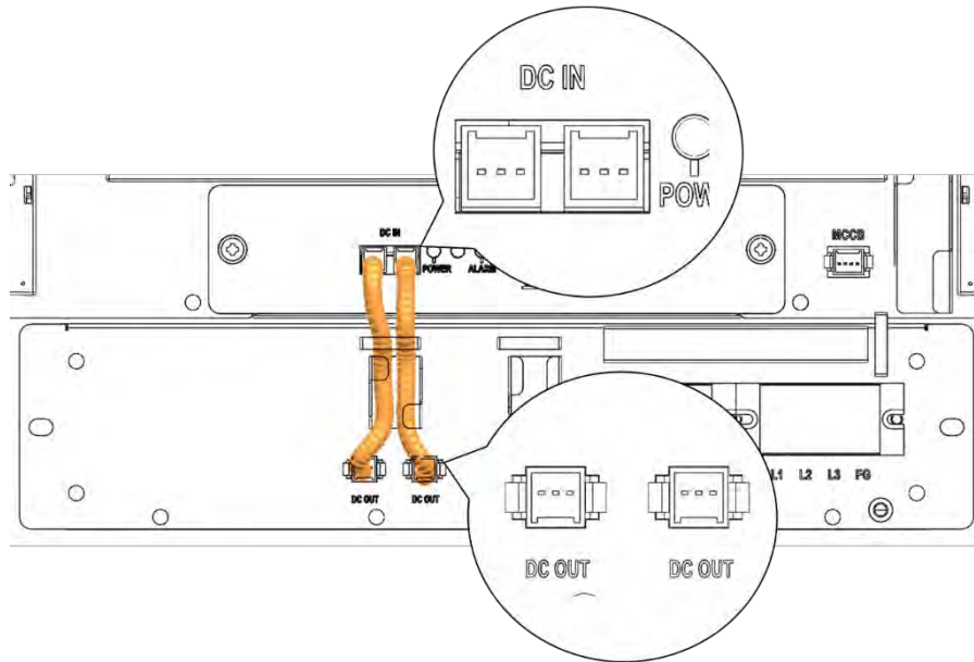
Figure 3-114: DC Power Cables from SMPS Assembly 3 Phase Type B to SMU
