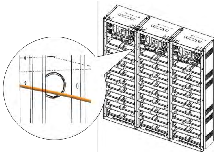
Figure 3-110: Pre-Punched Hole for Signal Cable
