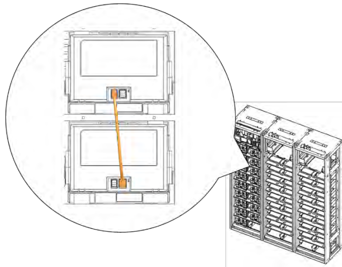
Figure 3-95: Module #2 to Module #3 Signal Cabling
