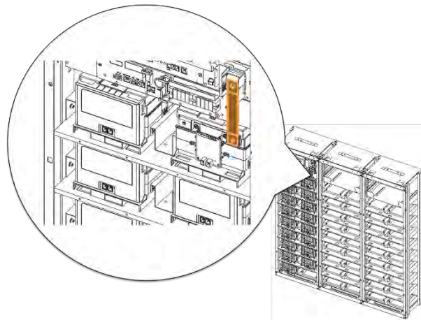
Figure 3-40: Connect SMU B- and Module #1 B-
