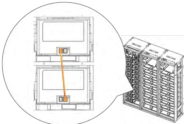
Figure 3-99: Module #6 to Module #7 Signal Cabling
