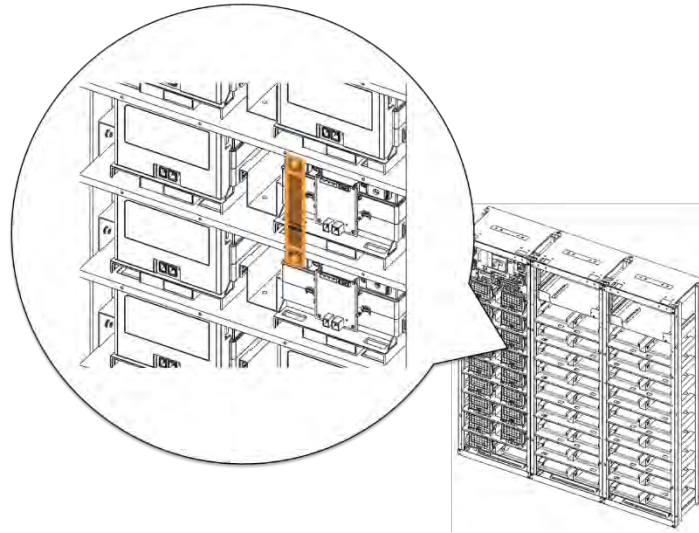
Figure 3-49: Connect Battery Module #3 B+ and Module #4 B-.
