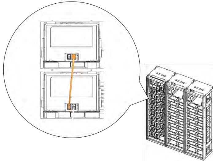
Figure 3-108: Module #15 to Module #16 Signal Cabling
