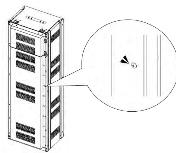
Figure 3-136: Front panel screws (eight)
