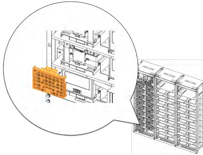
Figure 3-71: Reattach Battery Module #10's Front Cover
