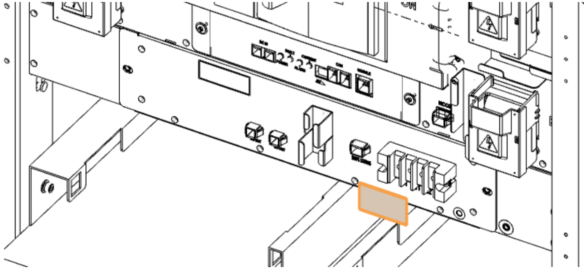
Figure 3-130: AC Input Terminals of SMPS Assembly 1 Phase Type B
