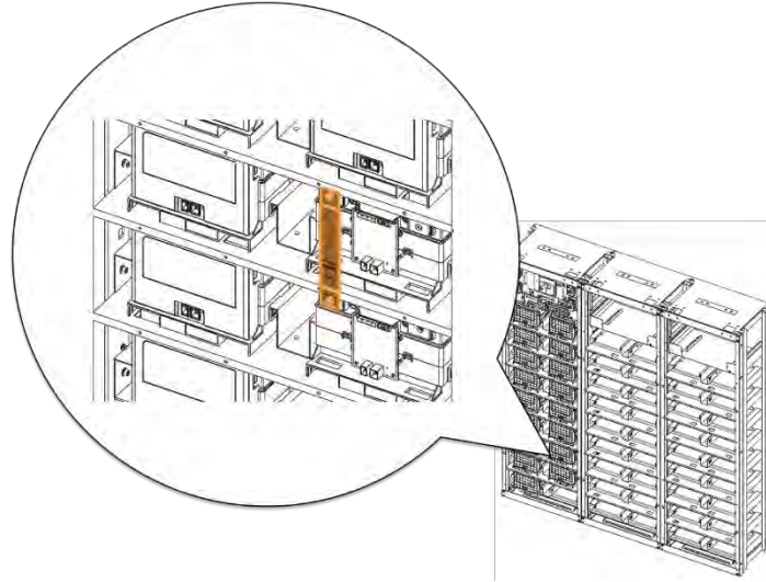
Figure 3-61: Connect Battery Module #7 B+ and Battery Module #8 B-
