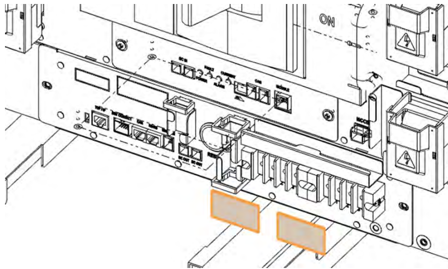
Figure 3-127: AC Input Terminals of SMPS Assembly 3 Phase Type A
