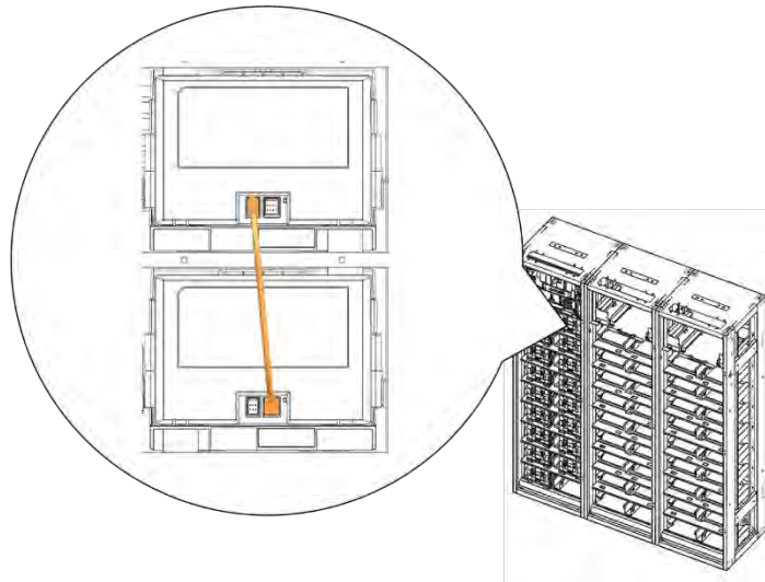
Figure 3-94: Module #1 to Module #2 Signal Cabling
