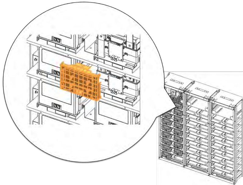
Figure 3-44: Reattach Battery Module #1's Front Cover
