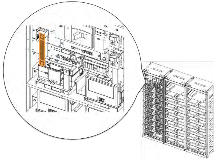
Figure 3-91: Connect SMU B+ and Module #17 B+.
