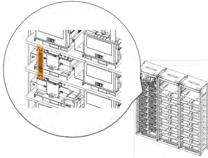
Figure 3-85: Connect Battery Module #15 B+ and Battery Module #16 B-.
