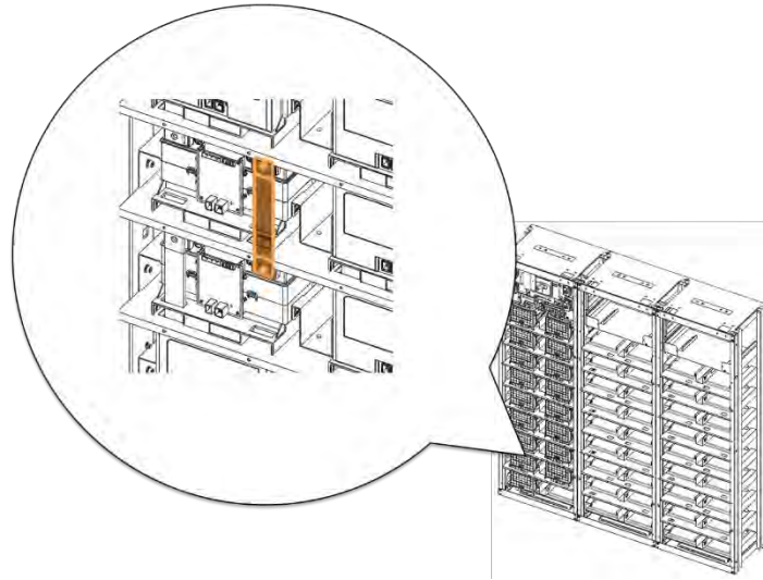
Figure 3-70: Connect Battery Module #10 B+ and Battery Module #11 B-.
