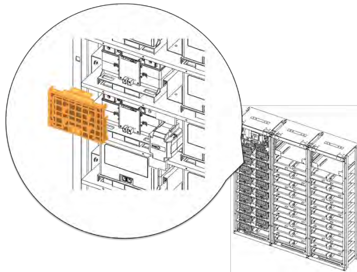
Figure 3-84: Remove Battery Module #16's Front Cover
