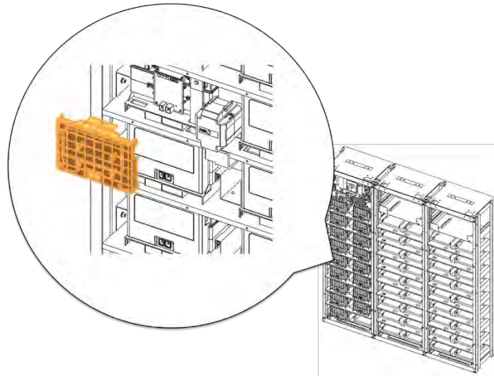
Figure 3-80: Reattach Battery Module #13's Front Cover
