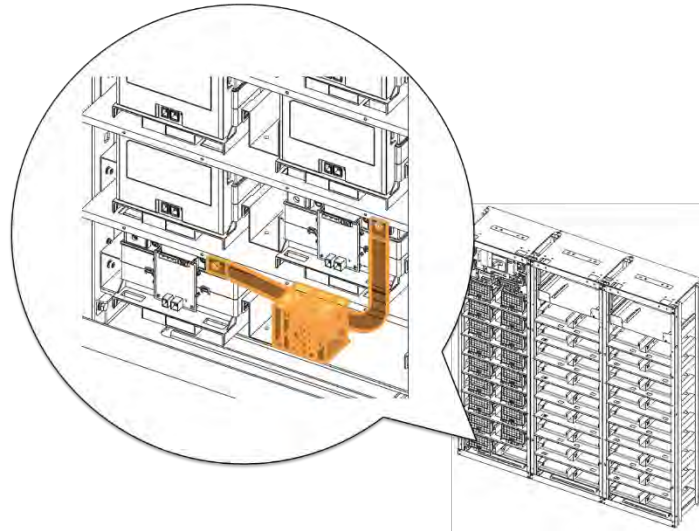
Figure 3-64: Connect Battery Module #8 B+ and Battery Module #9 B-.
