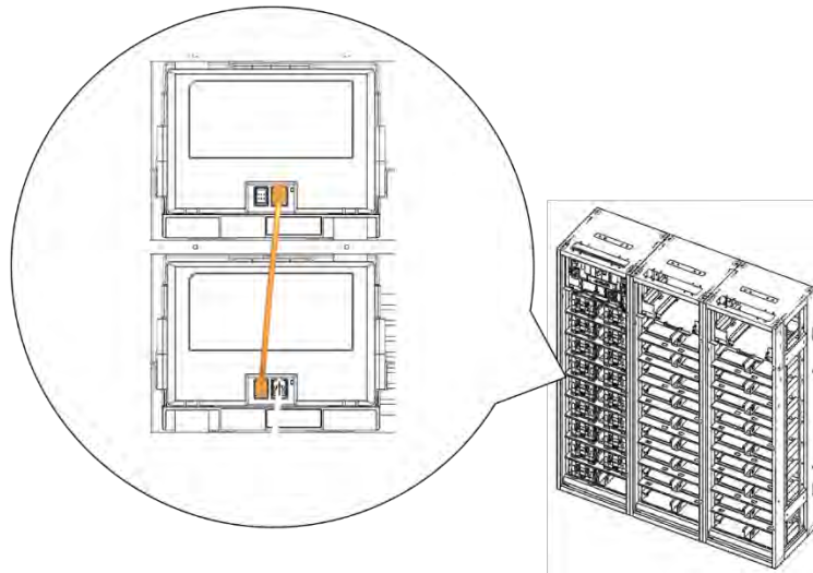
Figure 3-106: Module #13 to Module #14 Signal Cabling
