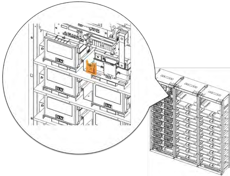
Figure 3-41: Restore SMU's B- Terminal
