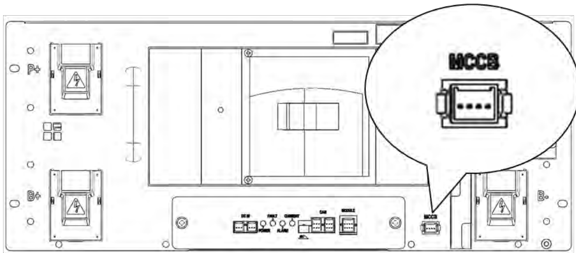
Figure 3-118: MCCB Extra Auxiliary Connection
