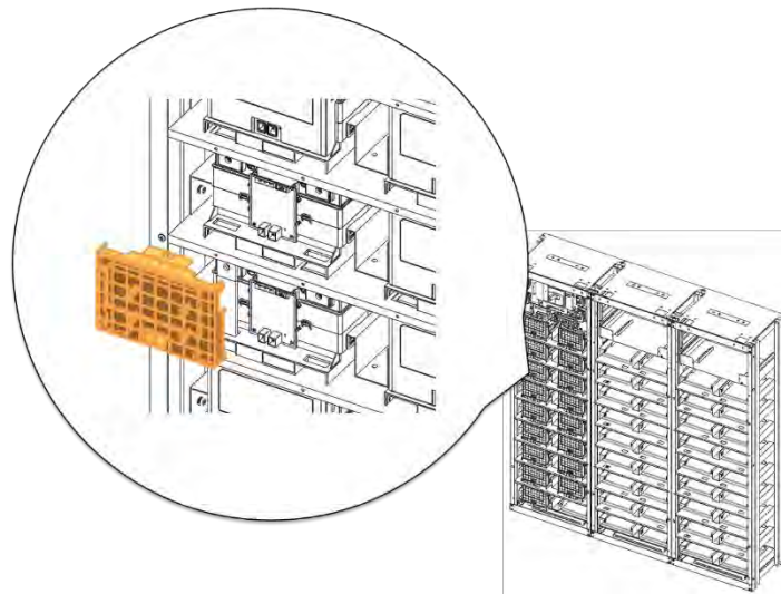
Figure 3-81: Remove Battery Module #15's Front Cover
