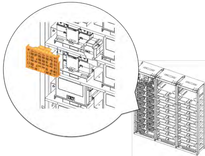
Figure 3-75: Remove Module #13's Front Cover
