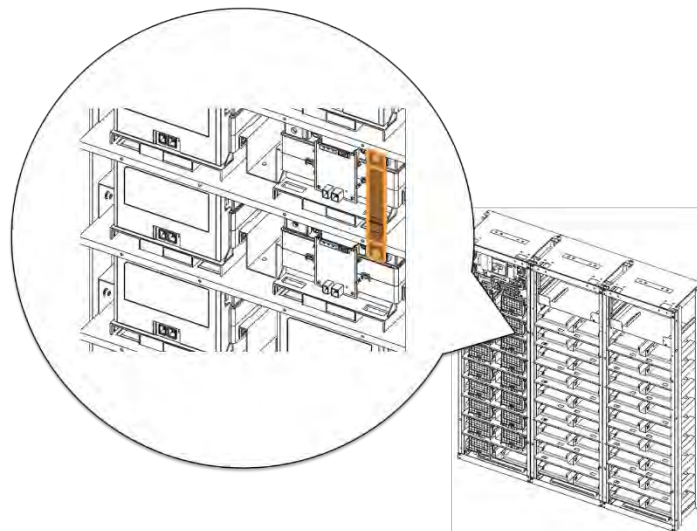
Figure 3-46: Connect Battery Module #2 B+ and Battery Module #3 B-.
