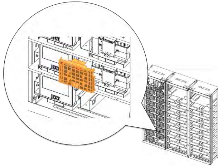
Figure 3-62: Reattach Battery Modules #7's Front Cover
