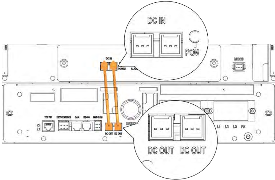
Figure 3-113: DC Power Cables from SMPS Assembly 3 Phase Type A to SMU
