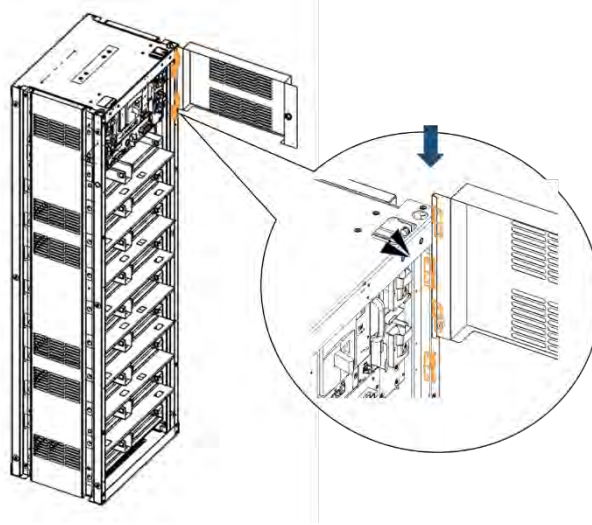
Figure 3-133: Reattaching the Front Door
