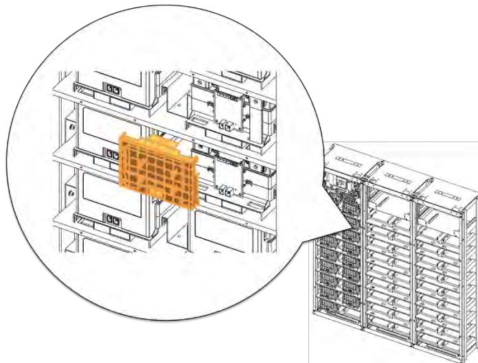
Figure 3-47: Reattach Battery Module #2's Front Cover
