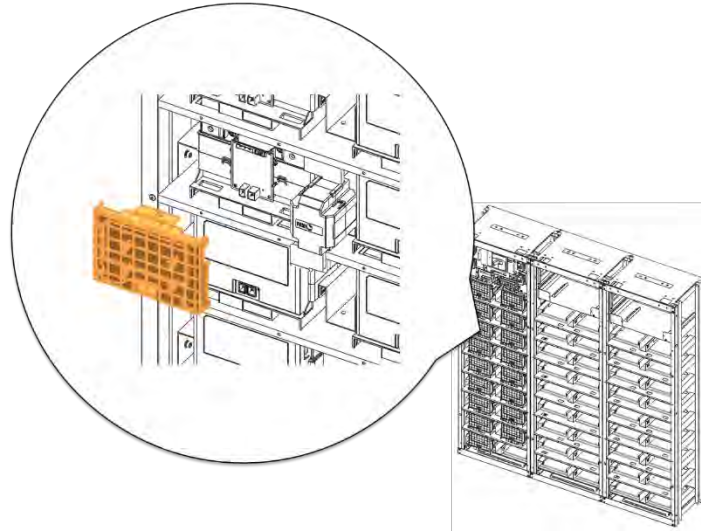
Figure 3-86: Reattach Battery Module #15's Front Cover
