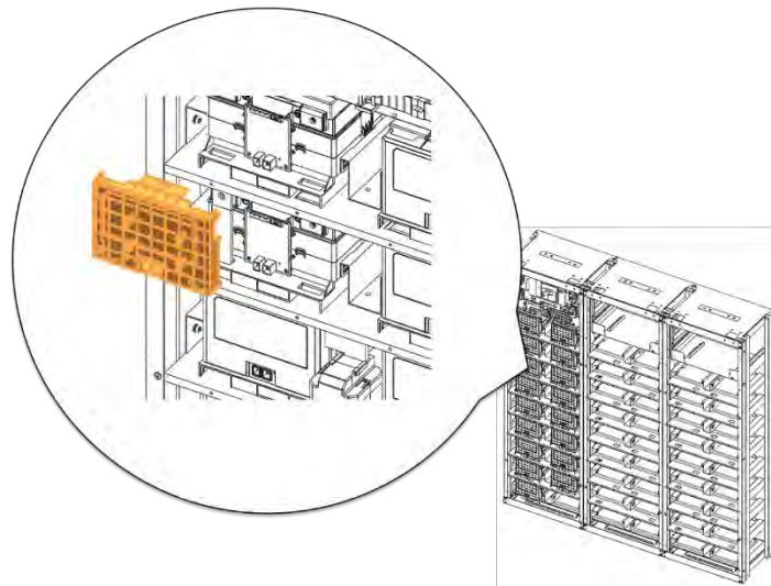
Figure 3-87: Remove Battery Module #17's Front Cover
