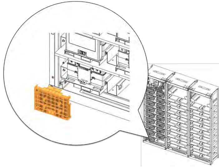
Figure 3-63: Remove Battery Modules #9's Front Cover
