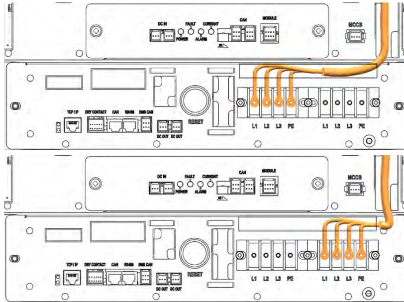
Figure 3-123: SMPS Assembly 3 Phase Type A - AC Input Terminals with Cables Attached
