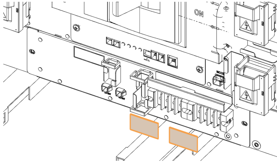
Figure 3-128: AC Input Terminals of SMPS Assembly 3 Phase Type B
