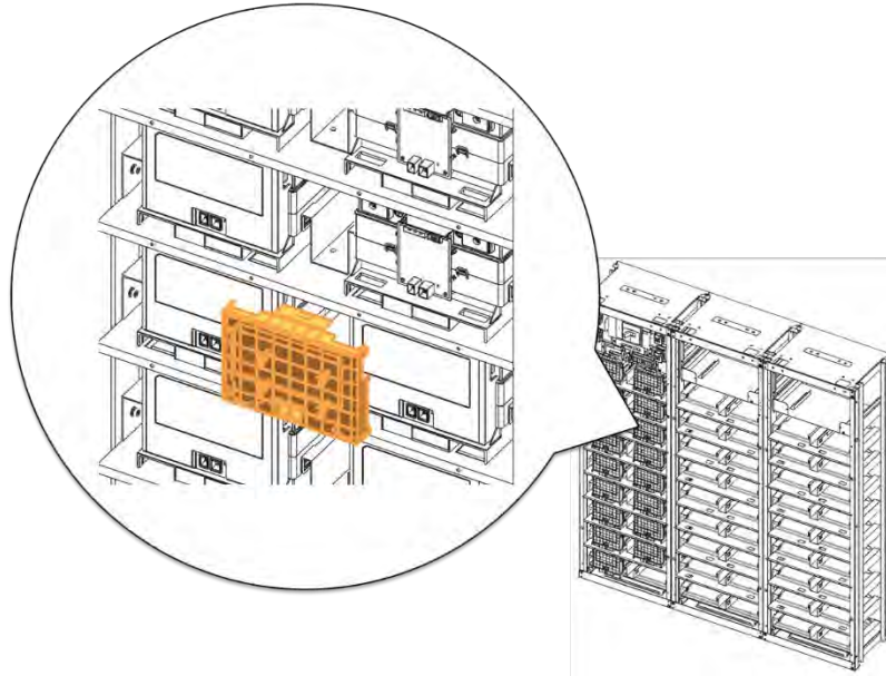
Figure 3-45: Remove Battery Module #2's Front Cover
