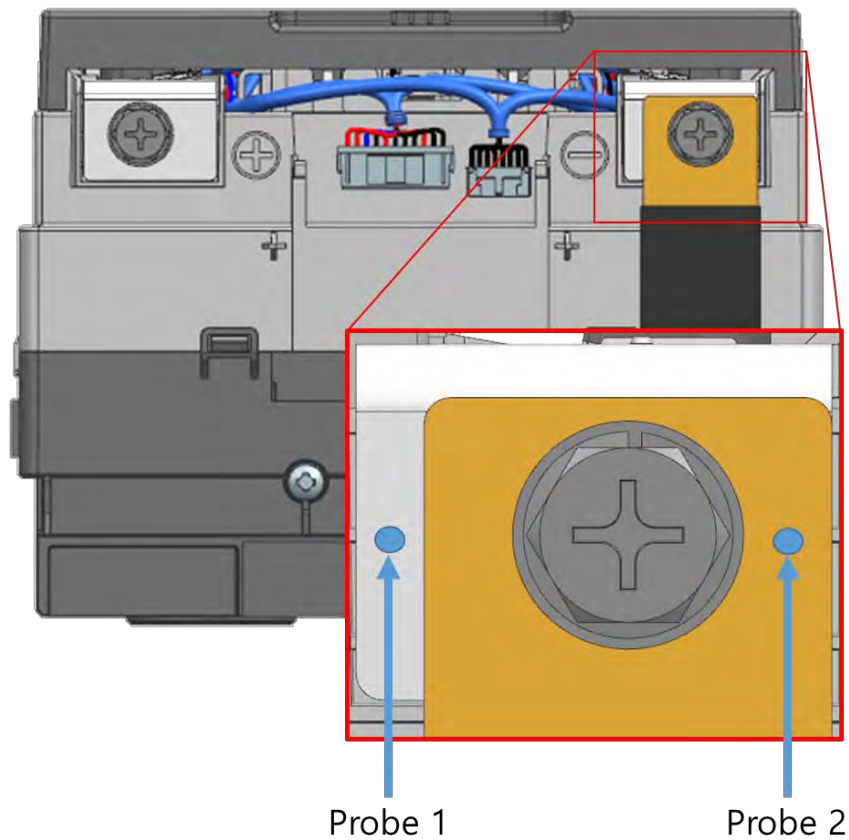
Figure 3-38: Contact Resistance Probe Points (Battery Module Terminal to Busbar)
