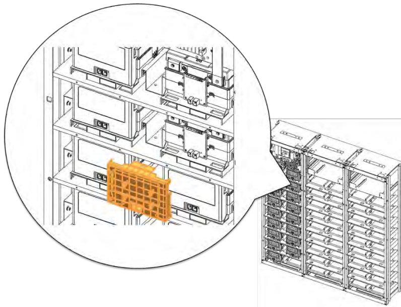
Figure 3-42: Remove Battery Module #2's Front Cover
