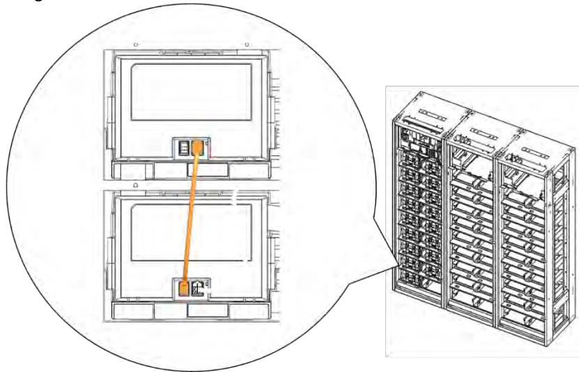
Figure 3-102: Module #9 to Module #10 Signal Cabling
