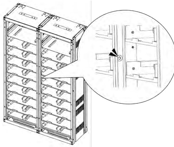
Figure 3-12: Holes on the sides of the rack (six)
