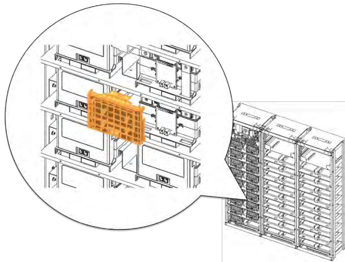
Figure 3-59: Reattach Battery Module #6's Front Cover
