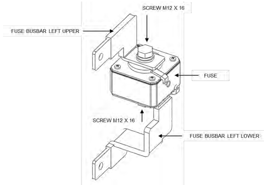
Figure 3-32: Fuse Busbar Left Assembly
