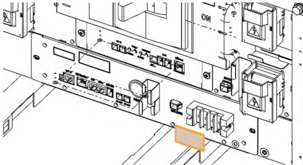
Figure 3-129: AC Input Terminals of SMPS Assembly 1 Phase Type A
