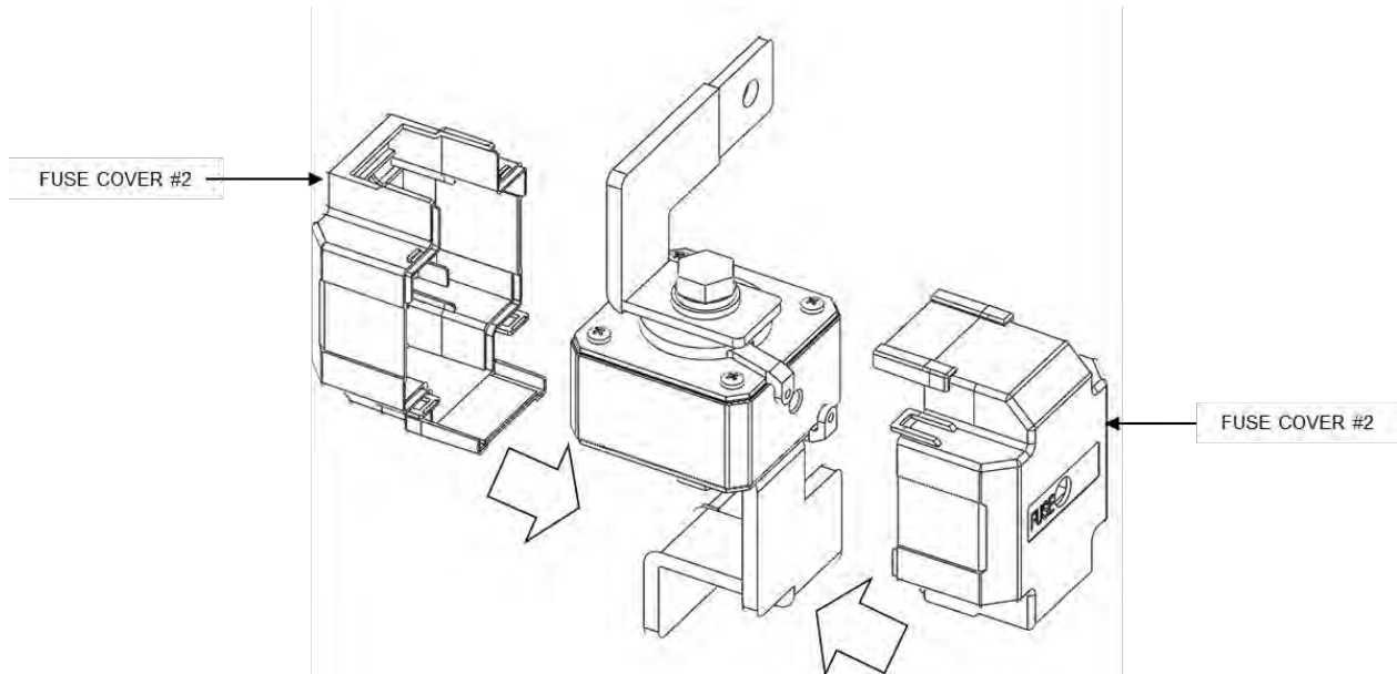
Figure 3-35: Fuse Busbar Right Assembly (Fuse Cover)
