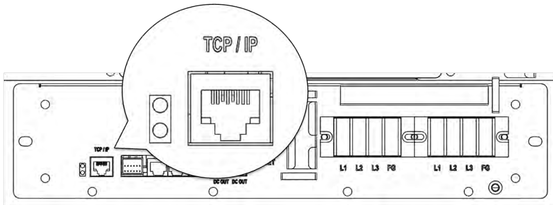
Figure 3-116: TCP/IP Cable Connection to SMPS Assembly
