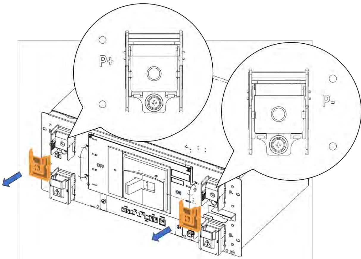
Figure 3-132: Connecting the DC Link High Current Terminals
