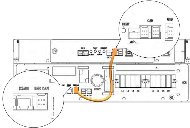
Figure 3-115: CAN Signal Cable Connection from SMPS Assembly 3 Phase Type A to SMU
