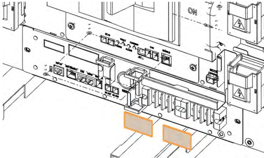
Figure 3-119: AC Input Terminals of SMPS Assembly 3 Phase Type A
