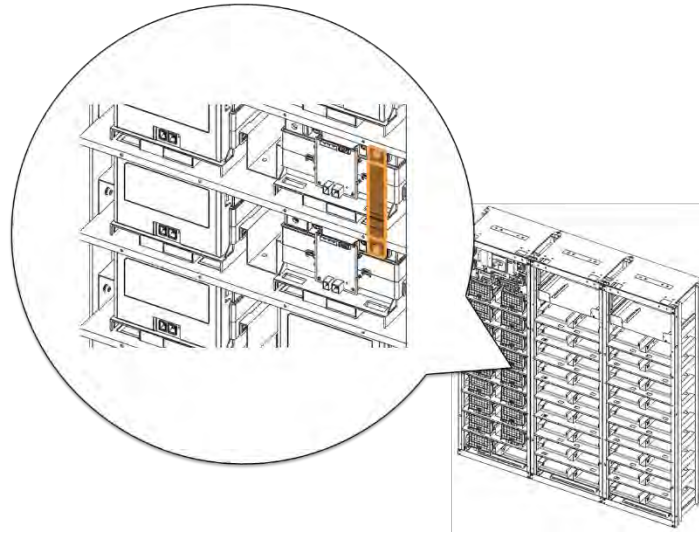
Figure 3-52: Connect Battery Module #4 B+ and Battery Module #5 B-.
