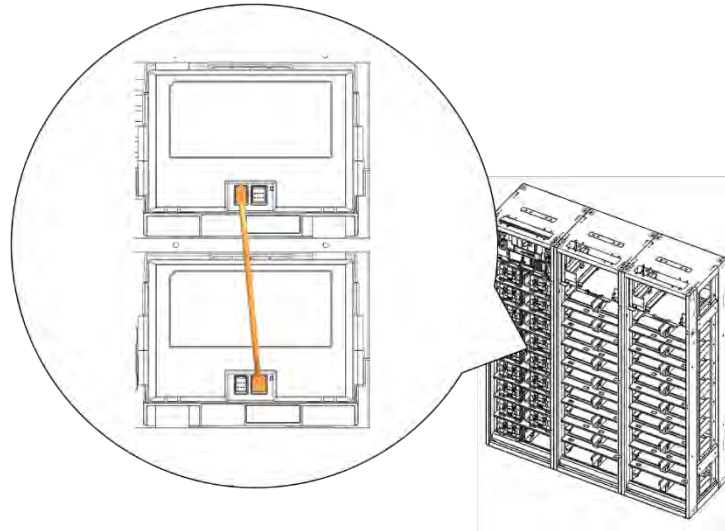
Figure 3-96: Module #3 to Module #4 Signal Cabling
