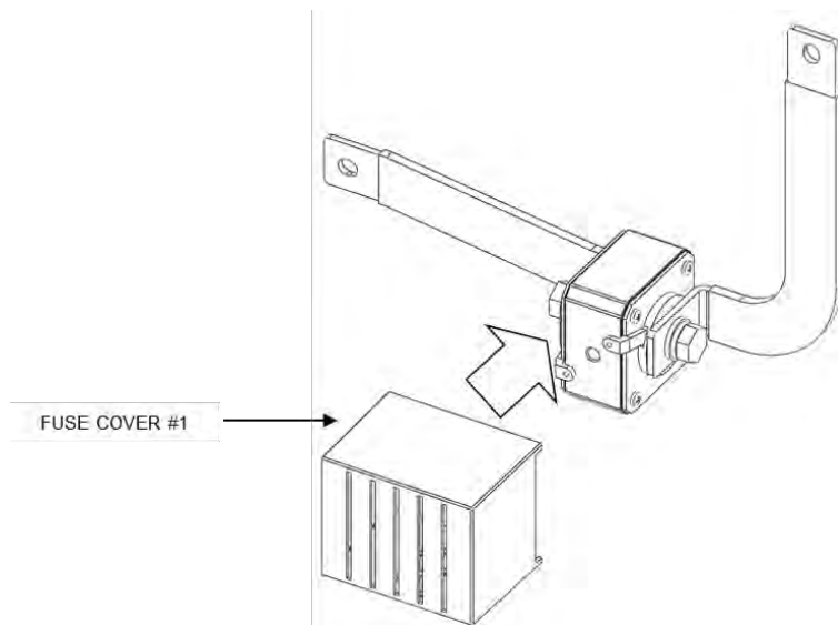
Figure 3-31: Rack Fuse Busbar Assembly (Fuse Cover)
