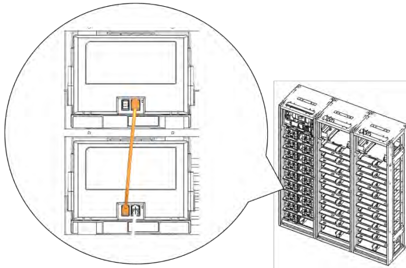
Figure 3-104: Module #11 to Module #12 Signal Cabling
