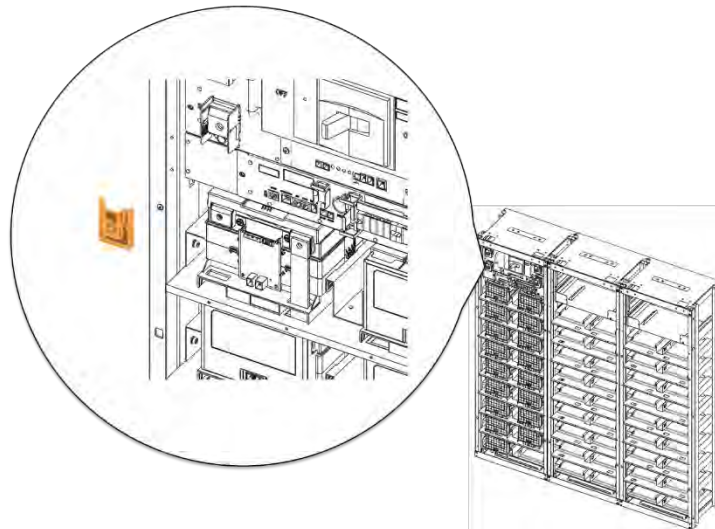
Figure 3-90: Remove SMU B+ Terminal Cover
