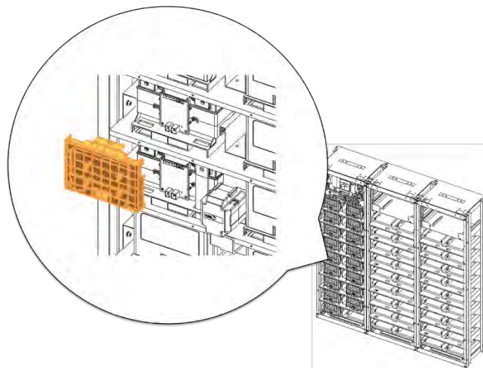
Figure 3-78: Remove Battery Module #14's Front Cover
