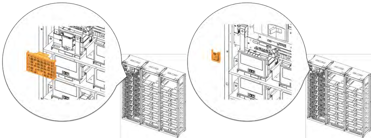
Figure 3-92: Reattach Battery Module #17's Front Cover and SMU B+ Terminal Cover
