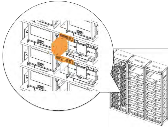
Figure 3-55: Connect Battery Module #5 B+ and Battery Module #6 B-.
