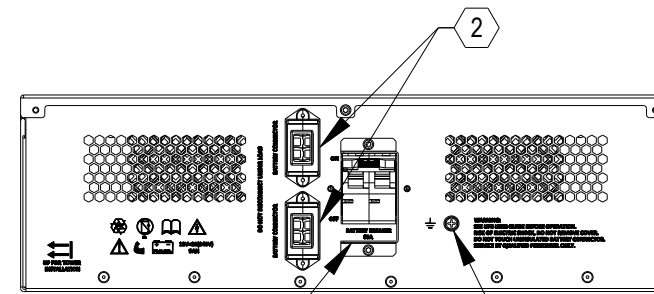
REAR VIEW
